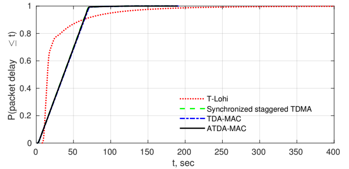
(b) Scenario 2: 100 nodes, 100 b/s channel, 64 bit packet length
