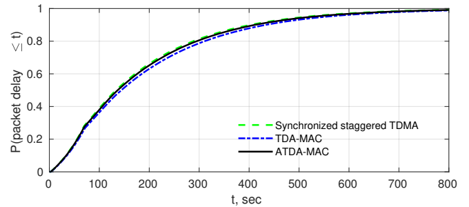
(b) Scenario 2: 100 nodes, 100 b/s channel, 64 bit packet length
