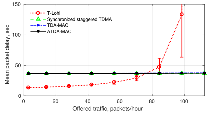
(b) Scenario 2: 100 nodes, 100 b/s channel, 64 bit packet length
