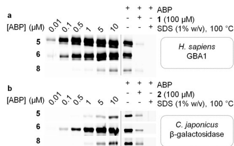
Fig. 2 Fluorescent labelling of recombinant H. sapiens GBA1 and C. japonicus \beta -galactosidase with ABPs 5 , 6 and 8 (left panel), and competition experiments with selective cyclohexenol inhibitors 1 or 2 (right panel). (a) GBA1 is potently labelled by 5 and 6 , but not 8 . All labelling was activity-based, indicated by competition experiments with GBA1 selective inhibitor 1 . (b) \beta -galactosidase is potently labelled by 5 , in an activity-based fashion.
