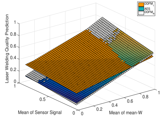
Fig. 6. Band width for the Fuzzy model surface that correspond to seam 'B'
