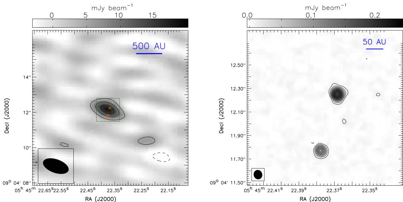
Fig. 1. Interferometric images of FU Ori (contour and grayscale). Left:– SMA 224 GHz image. Contour levels are 4.8 \text{ mJy beam}^{-1} ( 3\sigma ) \times [-2, -1, 1, 2, 3] . Right:– JVLA 29-37 GHz image. Contour levels are 10.8 \mu\text{Jy beam}^{-1} ( 3\sigma ) \times [-2, -1, 1, 2, 3, 4, \dots, 13, 14, 15] . Dashed contours present negative intensity. Cross and square in the left panel mark the locations of FU Ori and FU Ori S, which were obtained from the 2-dimensional Gaussian fits to the JVLA 33 GHz image. Green box in the left panel shows the field of view of the right panel. We assume a distance of 353 pc.
