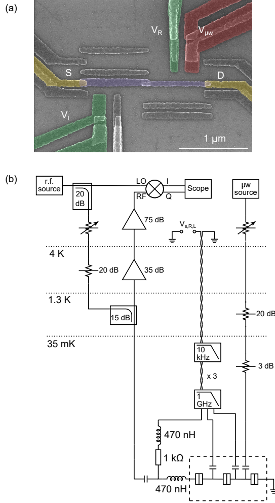
FIG. 3. Device and experimental wiring. a) False color SEM of SDD. Superconducting islands are in purple, normal state leads are in yellow. Electrostatic gates are highlighted in green (DC) and red (microwave frequencies). Uncoloured features are artifacts of the three angle evaporation process. b) Experimental wiring. The reflectometry circuit is shown on the left; d.c. wiring in the middle, with low temperature RC and Eccosorb filtering; and the microwave line on the right, with attenuation at 1.4 K and 35 mK.
