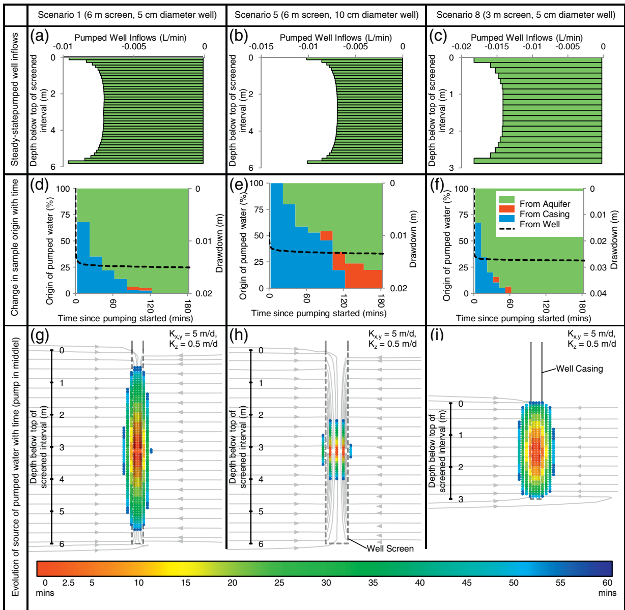
Fig. 3. Simulated pumped sample origin for Scenarios 1, 5 and 8 under ambient horizontal gradients. The first row shows the steady-state pumped well inflows. The second row shows the variation in pumped water origin with time compared with the simulated drawdown. The third row shows the temporal evolution of sample origin with the pump intake located at the middle of the screen. In all cases the pumping rate is 0.3 l/min. Particle color indicates time, arrowed lines indicate long-time pumping capture zone.
