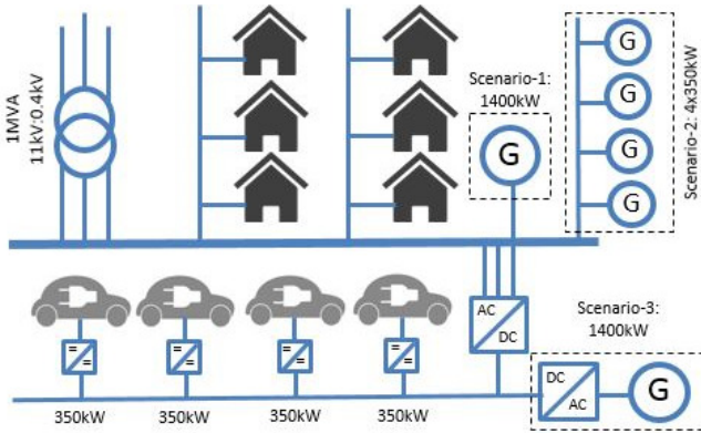
Fig. 1 HPC system topology with ac grid interface and possible connection options for CHP units.
