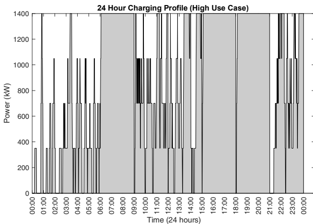
Fig. 5 High use case loading profile.
