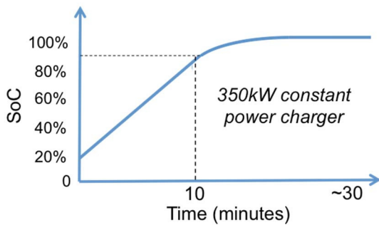
Fig. 2 Battery charging behavior model: constant power charging between 20%-90% SoC
