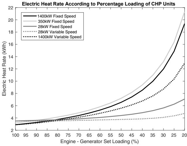
Fig.6 EHR curves per the percentage loading condition for 28kW, 350kW and 1400kW gas reciprocating gensets.
