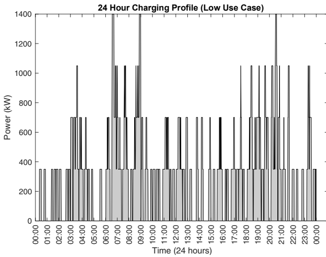
Fig. 3 Low use case loading profile.
