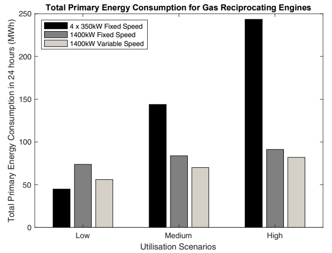
Fig. 7. Total primary energy consumption (natural gas) used in the operation of gas reciprocating engines for the charging of BEVs at an HPC station.
