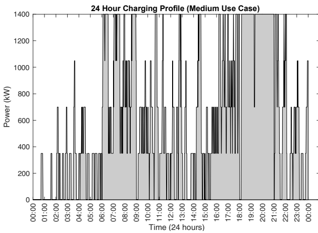
Fig. 4 Medium use case loading profile.
