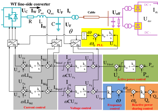
Fig. 2 Diagram of WT line-side converter control
