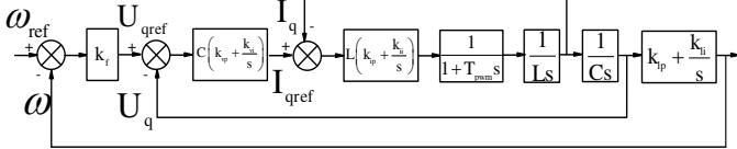
Fig. 6 Closed loop of PLL-based frequency control
