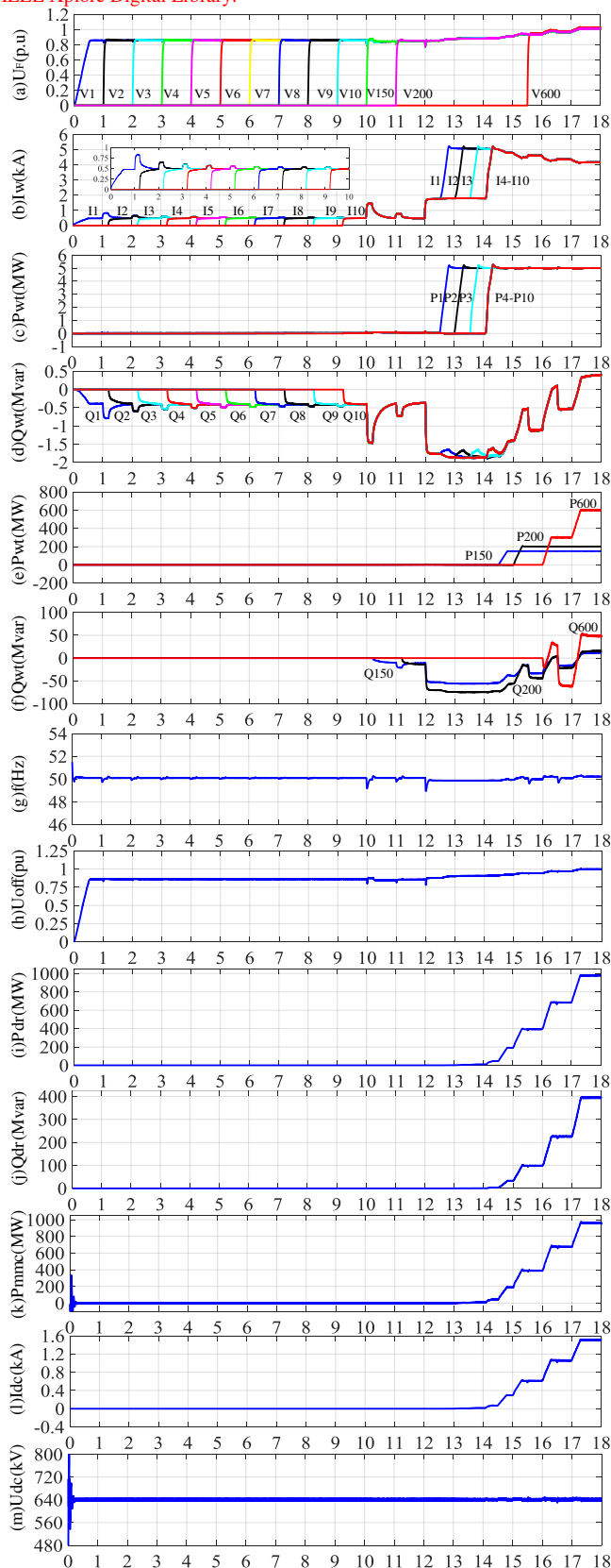
Fig. 8 Performance of start-up and synchronization: (a) WT voltage (RMS); (b) WT current (RMS); (c) WT active power; (d) WT reactive power; (e) aggregate WT power; (f) aggregate WT reactive power; (g) offshore frequency; (h) offshore voltage; (i) diode rectifier transmitted active power; (j) diode rectifier reactive power consumption; (k) onshore transmitted active power; (l) dc current; (m) dc voltage
