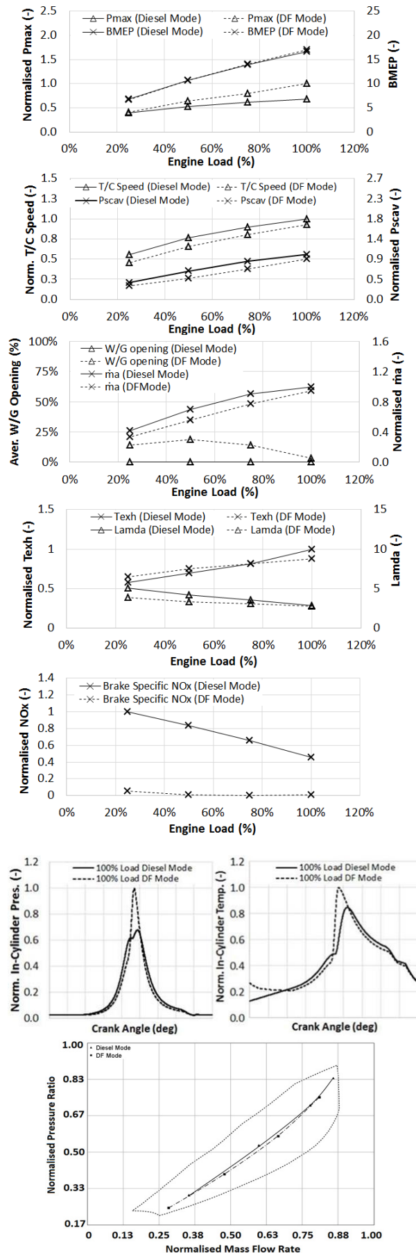
Fig.2 Simulation results at steady state conditions
