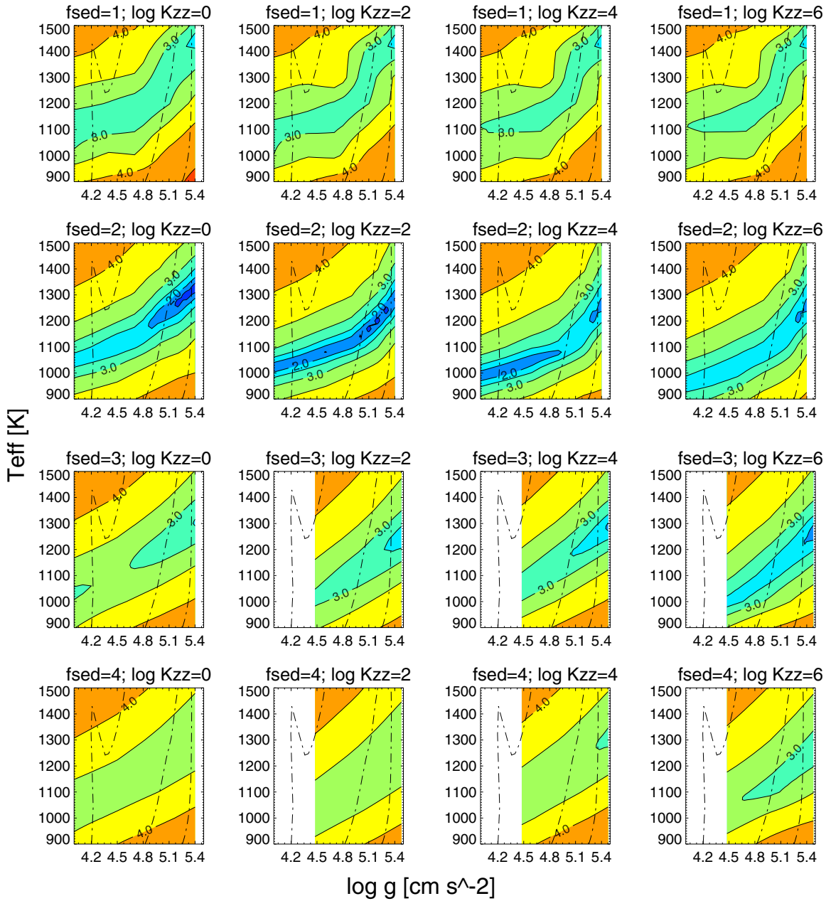
Figure 8. Contours of model fitting \log \chi^2 as a function of T_{\text{eff}} and \log g for the 16 combinations of f_{\text{sed}} and \log K_{zz} for WISE 0611–0410 A. The dot-dashed lines denote f_{\text{sed}} = 2 , \log K_{zz} = 0 objects with ages 0.1, 1, and 6 Gyr (left to right). The upturn in T_{\text{eff}} from \approx 1250 K to \approx 1450 K for the 0.1 Gyr model is caused by deuterium fusion in the cores of these objects. The contour levels and associated colors are the same in all panels. The \log K_{zz} = 0 model represents the equilibrium chemistry case. Note that the gravities for the f_{\text{sed}} = 3 and 4, \log K_{zz} = 6 do not span as wide of a range as the other model cases.
