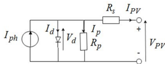
Fig. 2 PV cell circuit model.
