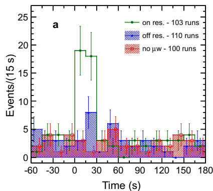
Fig. 2. Appearance data for the \bar{\text{H}} microwave experiment versus exposure time, with the microwaves applied at t = 0 . The two possible quantum jumps were each subject to 15 s bursts of microwaves, repeated over the 180 s duration of the trial. A trial consisted of forming antihydrogen, and then waiting an appropriate time (typically a second or so) to ensure that the excited states produced via reaction (1) had decayed to the ground state before commencing irradiation. There is a clear excess of counts in the two first time bins, indicating that the low- to high-field seeking transitions have been excited. With hindsight, the microwave power used meant that almost all the \bar{\text{H}} atoms were expelled from the trap during the first 15 s burst. The on-resonance (green), off-resonance (blue hatched) and no microwaves (red hatched) each consisted of around 100 trials.
