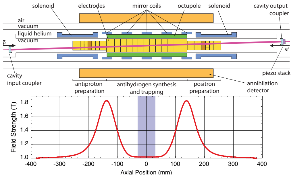
Fig. 1. Schematic illustration of the ALPHA2 apparatus used for the 1^3\text{S} - 2^3\text{S} experiment [1]. The various Penning trap electrodes are shown, including those for the \bar{p} and e^+ preparation regions, which are themselves fed by the catching trap and buffer gas accumulator respectively (see text). The extra solenoids provide confining fields for the charged particles in these regions. The neutral atom trap is comprised of the set of mirror coils and the octupole. A schematic of the laser cavity is shown. The 243 nm light enters from the left side and crosses the central region of the trap at an angle of 2.3^\circ . The annihilation detector is shown in block form (with its actual radial extent being larger than shown) and consists of a 3-layer silicon device, as explained further in the text.
