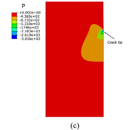
Fig. 9. Contour plots of (a) oxygen concentration ( \text{g}/\text{mm}^3 ), (b) opening stress (MPa) and (c) hydrostatic pressure (MPa) around the crack tip for fully coupled analysis ( K = 25.37 \text{ MPa}\sqrt{\text{m}} and loading time t = 3600 \text{ s} ).
