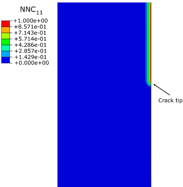
Fig. 8. Contour plot of oxygen concentration ( \text{g}/\text{mm}^3 ) around the crack tip for natural diffusion ( t = 3600 \text{ s} ).
