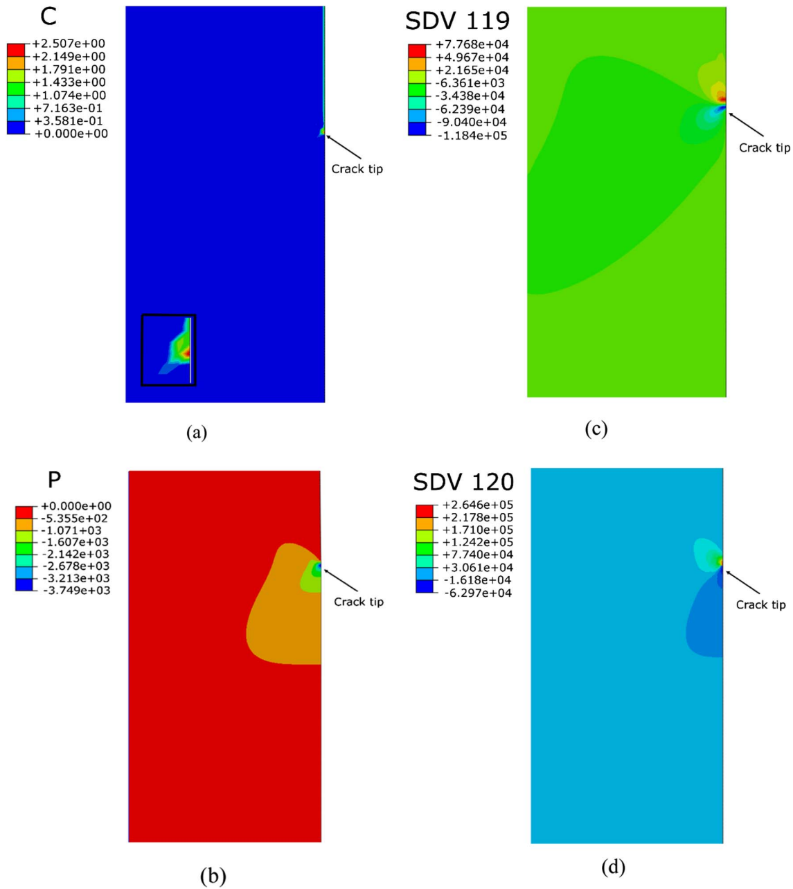
Fig. 6. The contour plots of (a) oxygen concentration ( \text{g}/\text{mm}^3 ), (b) hydrostatic pressure (MPa), (c) pressure gradient (MPa/mm) parallel to crack and (d) pressure gradient (MPa/mm) perpendicular to crack for sequential coupling analysis ( K = 25.37 \text{ MPa}\sqrt{\text{m}} and loading time t = 3600 \text{ s} ).
