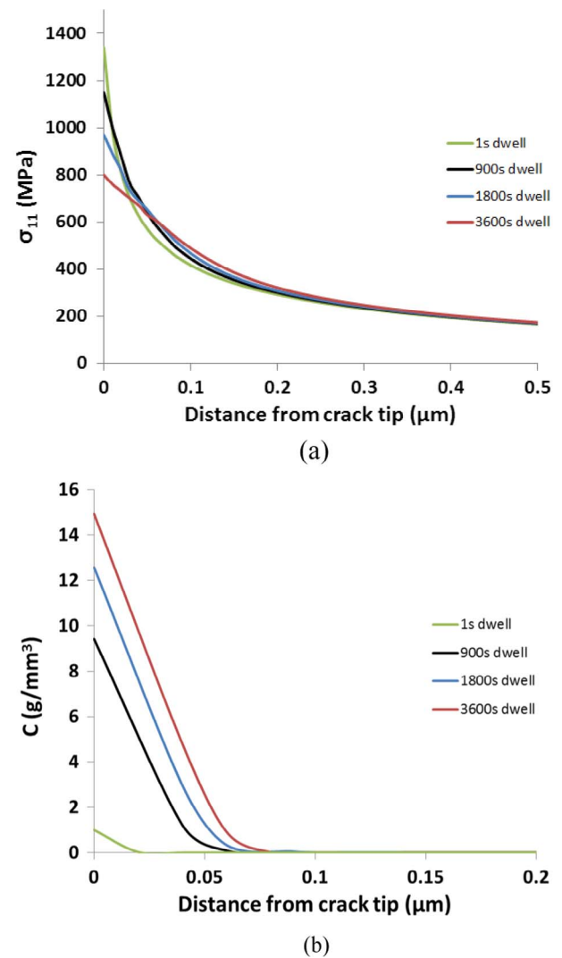
Fig. 11. Effect of dwell time on (a) crack opening stress and (b) oxygen concentration ahead of a stationary crack tip (loading time = 1 s, \Delta K = 25.37 MPa \sqrt{\text{m}} , load ratio R = 0 , dwell is superimposed on peak load).
