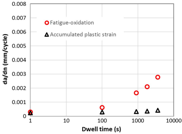
Fig. 14. Predicted fatigue crack growth rate in oxidation environment for different dwell times with \Delta K = 25.37 MPa \sqrt{m} ; Predicted crack growth rates in vacuum are also included for comparison.
