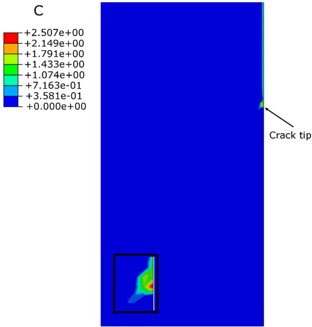
Fig. 7. Contour plot of oxygen concentration ( \text{g}/\text{mm}^3 ) around the crack tip for sequential coupling using ABAQUS' own procedure ( K = 25.37 \text{ MPa}\sqrt{\text{m}} and loading time t = 3600 \text{ s} ).
