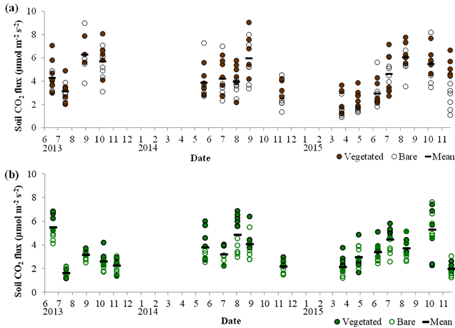
Figure 4. Variations in soil CO 2 efflux for each measurement event for combined grass and bracken plots, results separated for vegetated (● filled circles) and bare (○ open circles) soil plots at (a) the forest and (b) the grassland study sites ( n = 6).
