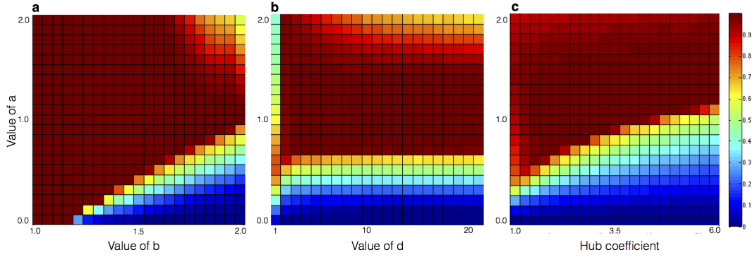
Figure 5: Varying affinity. In all plots the affinity parameter is varied from 0 to 2 in increments of 0.1. In plot (a), b is varied from 1 to 2 in increments of 0.05. In (b), d is varied from 1 to 21. In (c), \sigma is varied from 1 to 6 in increments of 0.25.
