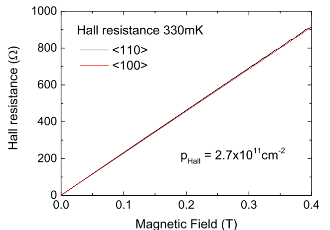
FIG. 2. Hall resistance for two orientations at 330 mK demonstrating that the carrier density is isotropic.
