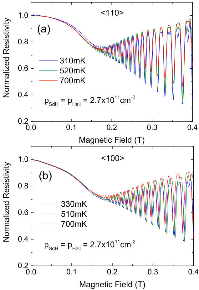
FIG. 3. Low temperature magnetoresistance curves for the two crystallographic orientations (a) \langle 110 \rangle and (b) \langle 100 \rangle , plotted on the same vertical scale to highlight the difference in damping (due to effective mass and scattering parameters).
