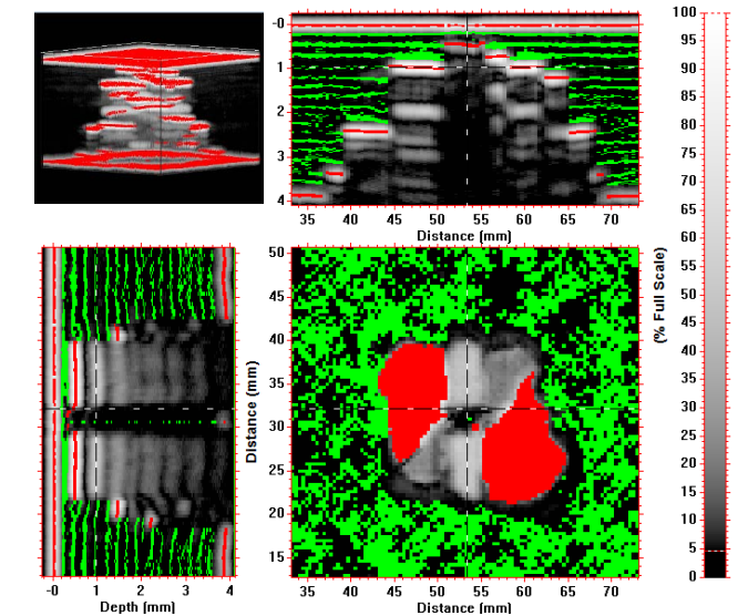
Fig. 12. 7.5-MHz immersion scan of impact damage in a 4-mm-thick composite with 0.25-mm ply spacing. Instantaneous amplitude is plotted in grayscale (right) with overlaid ultrasound-derived coding for front- and back-surfaces (red), delaminations (red), and inter-ply resin layers (green). Bottom-center is an in-plane C-scan slice 1-mm deep, whilst bottom-left and top-center images are B-scan slices at locations shown by black/white dashed lines on the C-scan. Top-left is a pseudo 3-D image with front, back, and delaminations showing red.
