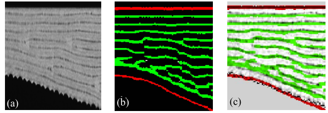
Fig. 9. Wedge specimen containing ply-drops, made from 0.189-mm plies and incorporating 0.04-mm resin layers. (a) X-ray CT slice. (b) Ultrasound-derived front-surface (red), back-surface (red), and resin-layer (green) locations (c) overlaid on X-ray CT data. The ultrasound scan used a 38-mm spherical-focus 7.5-MHz probe.
