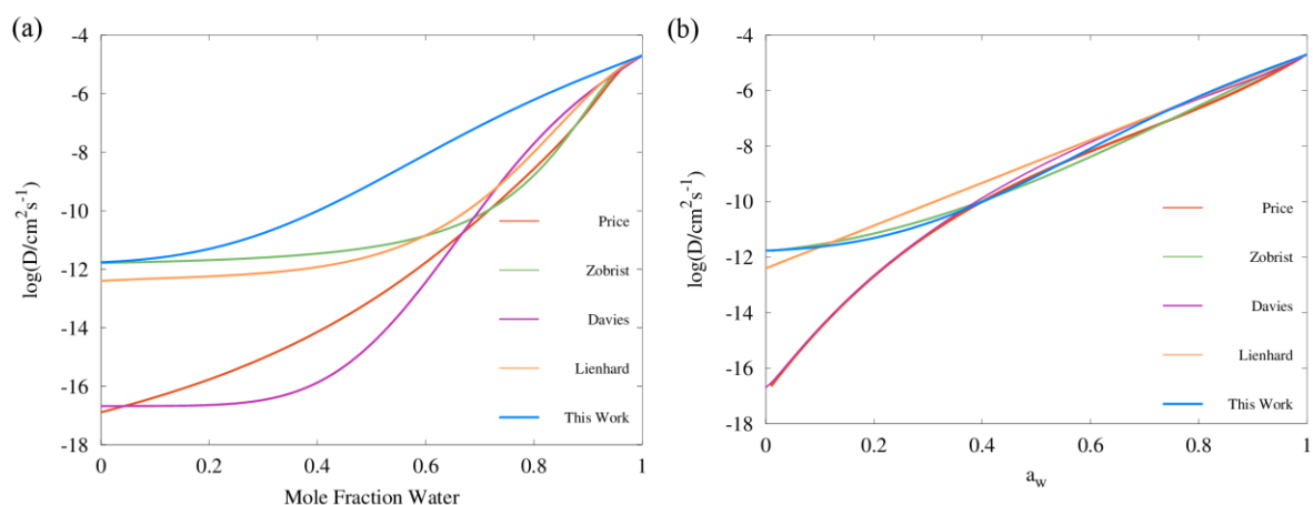
Figure 6. Comparison of diffusion coefficient parameterisations for sucrose aerosol plotted in (a) mole fraction space, and (b) water activity space: mean trend of Vignes functions (ideality assumed, with cubic treatment of \alpha coefficients) simulated with Fi_PaD, as shown in Figure 4a (Blue); Third order polynomial parameterisation of D_{wat}(a_w) in log space by Price et. al. 59 , converted to mole fraction using the AIOMFAC model; Vogel-Fulcher-Tammann (VFT) parameterisation by Zobrist et al. 6 to RH step experiments in an Electrodynamic Balance (Green); Temperature dependent Vignes functions (with binomial expansion of \alpha coefficients) fit to RH step experiments in an Electrodynamic Balance by Lienhard et al. 26 (Orange); Temperature independent Vignes functions (with cubic treatment of \alpha coefficients) fit to isotope exchange experiments by Davies et al. 30 (purple).
