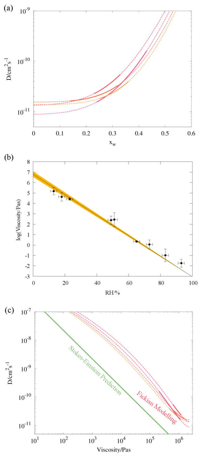
Figure 8: Stokes Einstein deviations of water diffusion in ternary aerosol containing sucrose, malonic acid and water. (a) As in Figure 4a, composition dependent diffusion coefficients fit to four radius responses using Fi-PaD (further details can be found in Table 2). (b) Single particle viscosity measurements, with a loglinear parametrisation. (c) Combination plot of data from (a) and (b) showing correlation between D and \eta . A comparison of the Stokes-Einstein predicted diffusivity for malonic acid (green) is also provided in panels (b) and (c).
