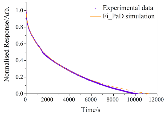
Figure 1. Example Fi-PaD fit to the response in size of a viscous droplet following a change in gas phase RH, monitored through the shift in a single WGM. The droplet is composed of a ternary aqueous solution of glucose and sucrose (solutes with mass ratio 1:1) following a step decrease in RH from 20 to 5 %. Model parameters are D_{w,org} = -11.42 , C = -9.71 , initial radius = 5205 nm.
