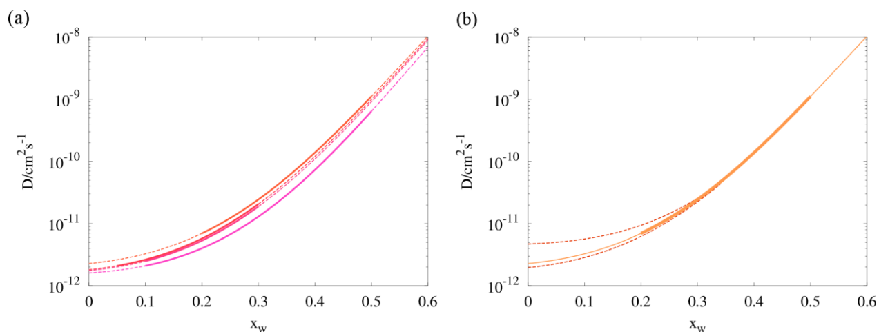
Figure 4. (a) Composition dependent diffusion coefficients estimated from four RH transitions in binary aqueous/sucrose droplets. Solid lines indicate the mole fraction range within which the model was evaluated, dashed lines represent the Vignes extrapolations. (b) Isolation of the 50-20% RH transition (“top-most” curve in panel a) showing the error envelope in the region 0 < x_w < 0.35 , as determined by equation (9) (red dotted lines). Exact values of the uncertainties in D_{w,org} for all four transitions may be inspected in Table 1.
