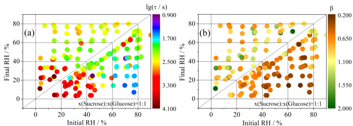
Figure 3. (a) Exponential folding time, \tau , of particle radius responses of ternary sucrose/glucose particles (1:1 mass ratio) to 172 step changes in RH, mapped over initial and final values. (b) The stretched exponential parameter, \beta , extracted for the same transitions by allowing it to vary during the fitting process.
