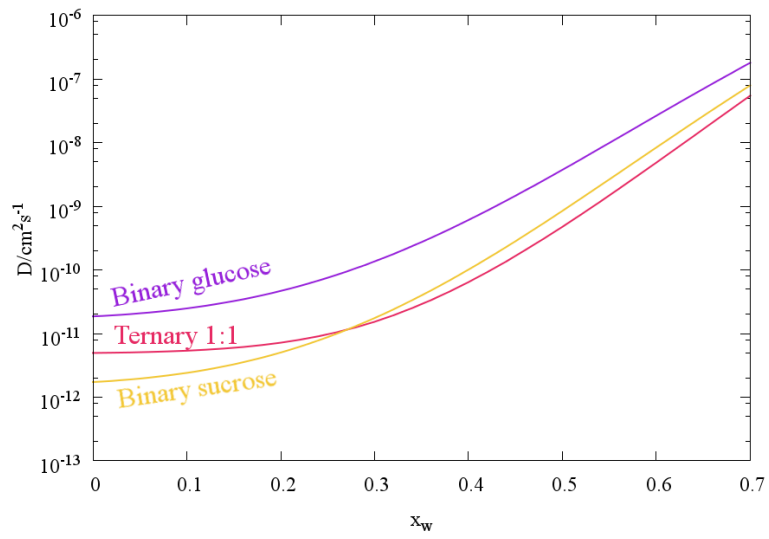
Figure 5. Mean composition dependent diffusion coefficient parametrisations for binary and ternary saccharide aerosol (as in Figure 4a). Each curve is produced from the mean D_{w,org} and C values of the transitions tabulated in Table 1.
