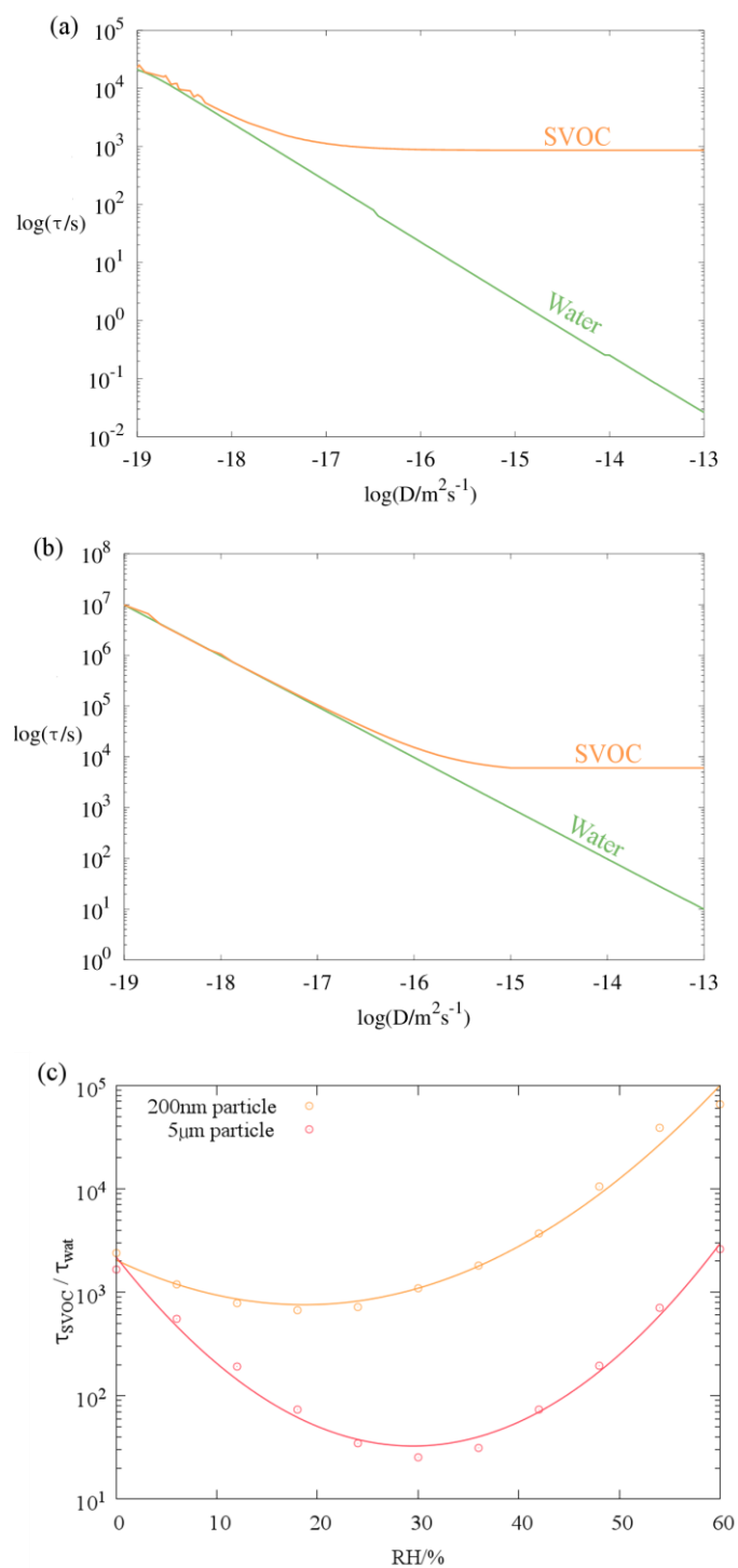
Figure 2. Concentration equilibration e-folding timescales, as determined from the model of Mai et al., for a hypothetical SVOC and water calculated over a wide range of bulk phase diffusion coefficients D typical for the volatile component. (a) 200nm radius particle; (b) 5μm radius particle. (c) The ratio of the two timescales at RHs below 60%, assuming that D_{SVOC} follows the Stokes-Einstein relation whereas D_w varies sigmoidally with RH (see main text).
