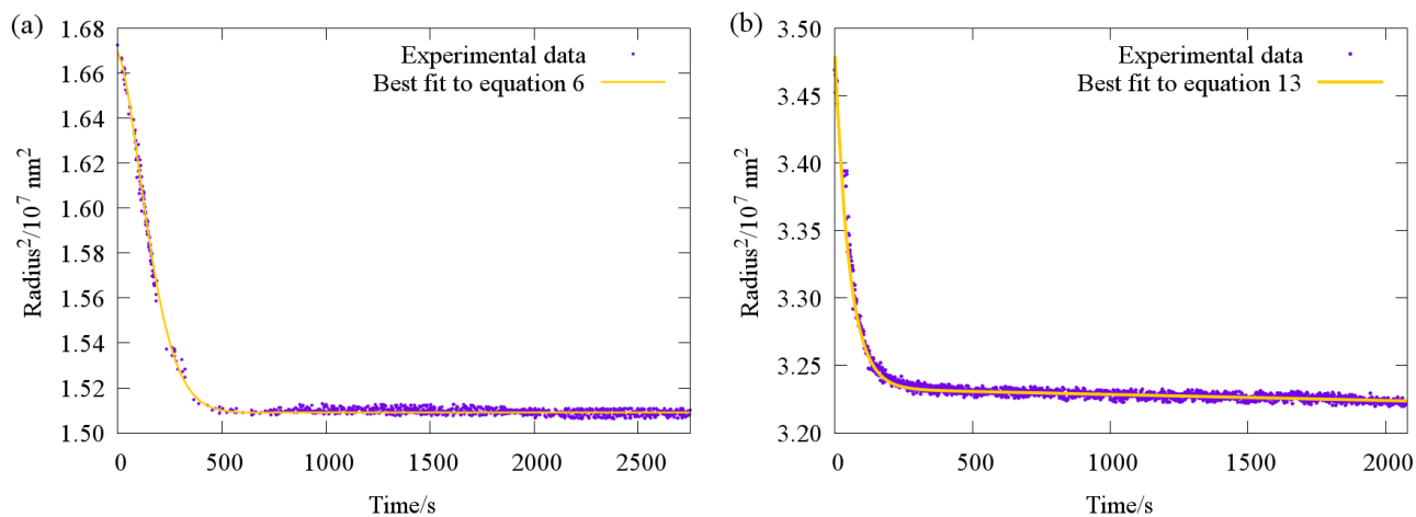
Figure 7. Typical evaporative profile (purple points) for ternary aerosol with (a) two involatile components (sucrose and glucose), and (b) one volatile and one semivolatile component (sucrose and malonic acid). Comparison with fit functions (yellow lines) based on the stretched exponential equations (6) and (13) are also shown.
