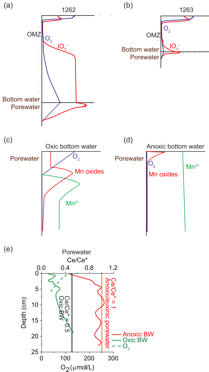
Figure 1. Expected iodate depth profiles in the water column and pore water for Sites (a) 1262 and (b) 1263, (c and d) Mn 2+ and Mn oxides depth gradient, and (e) Ce/Ce* profile in pore water under different redox conditions. Data for Figures 1a and 1b are from Rue et al. [1997] and Kennedy and Elderfield [1987]. Figures 1c and 1d are modified from Schenau et al. [2002] and Reitz et al. [2006]. The red line in Figure 1e represents the Ce/Ce* trend in sta10, a California margin site; the solid green line denotes the Ce/Ce* record in MC64, a site from the Nazca Ridge off Peru; and the dashed green line is the dissolved O 2 concentration in pore water at the same site [Haley et al. , 2004]. The red bar in Figure 1d is defined as Ce/Ce* = 1, and the grey bar as Ce/Ce* = 0.5. Ce/Ce* values to the left of the grey bar are typical in oxic pore water, while values between the red and gray bars suggest suboxic pore water, as is shown in Figure 2.
