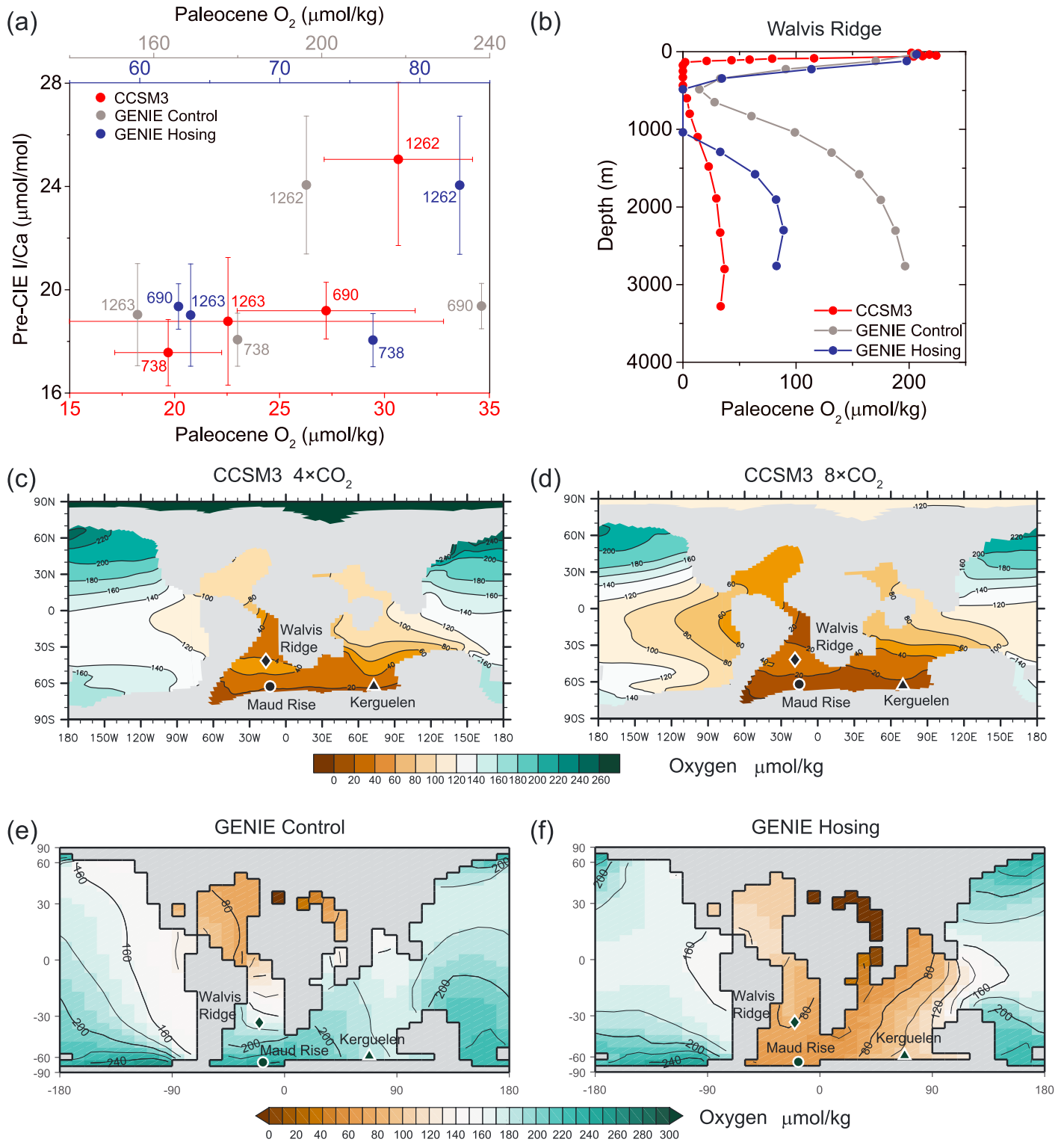
Figure 3. (a) Pre-CIE average N. truempyi I/Ca values at each site are plotted against modeled bottom water O 2 in the late Paleocene by CCSM3 [Winguth et al. , 2012] and two simulations by cGENIE (i.e., control and hosing). The error bars of pre-CIE I/Ca values stand for the standard deviation of those values, and those of modeled bottom water O 2 by CCSM3 represent the O 2 levels approximately 500 m above or below the paleodepth of each site. (b) Modeled O 2 concentrations through the water column at Walvis Ridge in the late Paleocene by CCSM3 and cGENIE. (c and d) Modeled global seafloor oxygen levels with atmospheric pCO 2 of ×4 and ×8 PAL in the late Paleocene by CCSM3. (e) Simulated global seawater O 2 levels at ~2000 m by cGENIE under the condition of ×3 CO 2 in the default late Paleocene (control experiment), with the symbols of diamond, circle, and triangle representing site locations of 1262 and 1263, 690, and 738, respectively. (f) Same settings as Figure 3e except adding fresh water at high-latitude South Atlantic Ocean (hosing experiment).
