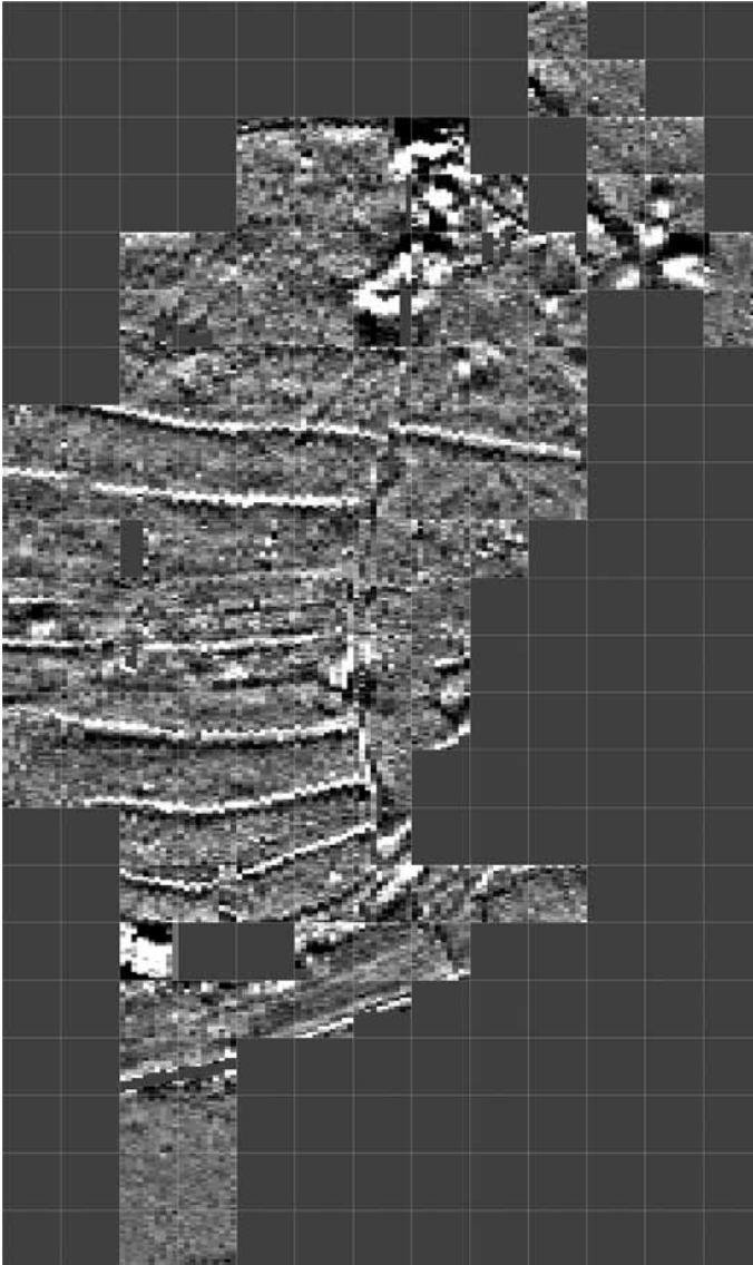
Figure 5.4: Geophysical results (photo Çaltılar Archaeological Project [ÇAP]).
