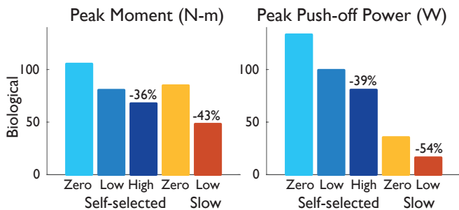
Fig. 7: Peak moment and push-off power produced by Subject B's ankle for different assistance levels. With greater assistance, the biological ankle provided less moment and power near push-off. Percentage decreases compared against Zero are at maximum -43% for moment and -54% for power.
