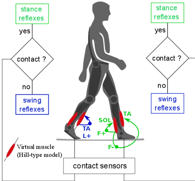
Fig. 1: Schematic view of the ankle module based on the reflex walking model from H.Geyer. Ground sensors are used to detect whether the limb is on stance or swing phase. Then, depending on whether the limb is in contact with ground or in swing, different reflex rules are generated, stance reflexes in green and swing reflexes in blue (Table 1 in [5] shows the different reflex loops acting depending on the gait phases). Here only the soleus and tibialis muscle modules are used. During stance, a positive force feedback ( F+ ) increases the tension in the soleus muscle, and a negative force feedback ( F- ) decreases the tension on the tibialis anterior to prepare for push off. During the entire gait cycle, a positive length feedback ( L+ ) tries to return the tibialis anterior muscles to a predefined length. Figure inspired from [10].
