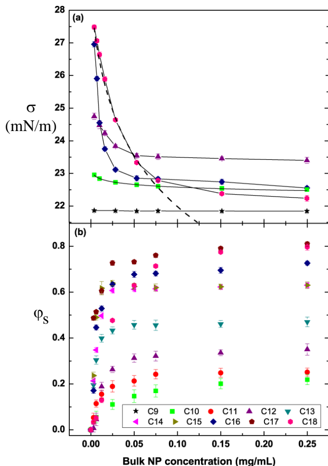
Fig. 15 (a) Liquid-vapor NP solution surface tension \sigma as a function of bulk dodecanethiol ligated Au NP concentration for selected n-alkane solvents. Solid line: guide to eye. (b) Surface concentration \phi_s , deduced from Eq. (33), as a function of bulk NP concentration. Reprinted (adapted) with permission from [31], © (2011) American Chemical Society.
