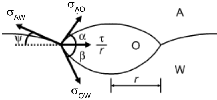
Fig. 20 Oil droplet (O) of lateral radius r at the air(A)/water(W) surface with interfacial tension \sigma_{ij} , between two phases i and j , and line tension \tau . The angles \alpha , \beta and \psi are defined in the figure.
