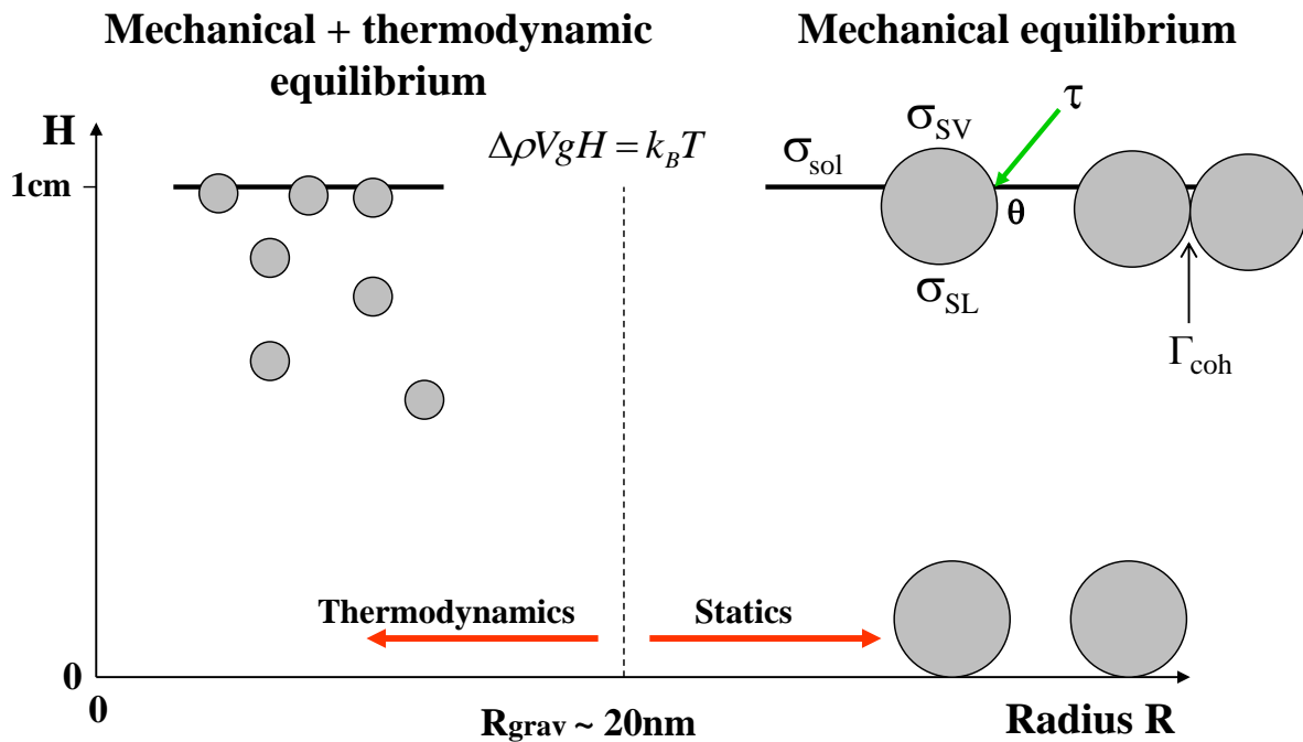
Fig. 11 Schematic of size-dependent colloidal particle behavior at liquid-vapor surfaces. When R \gg R_{grav} ( R \ll R_{grav} ), described in Sec. 3.1.1 (Sec. 3.1.2), colloidal particles sediment out of solution (remain suspended in solution).
