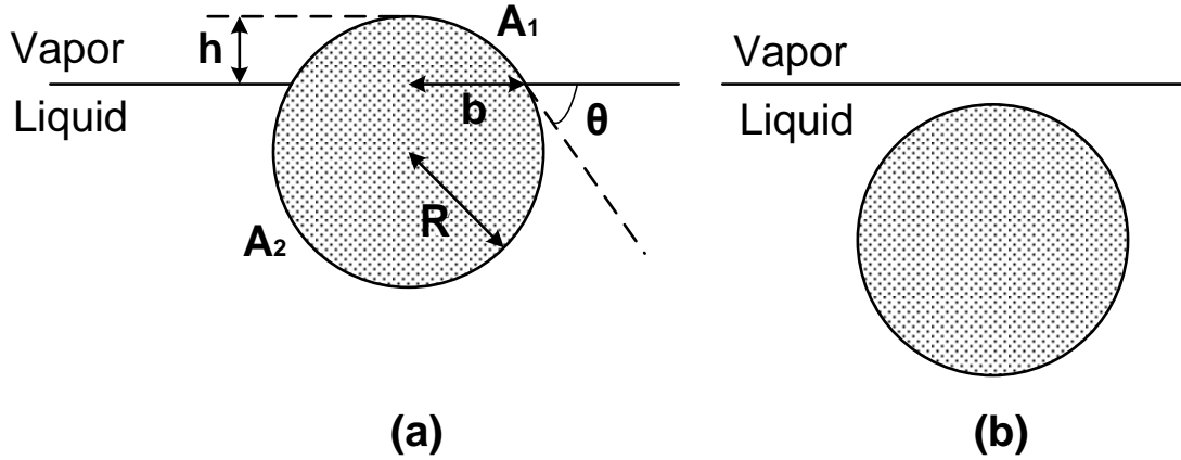
Fig. 12 (a) Spherical colloidal particle of radius R , at a liquid-vapor surface, with protrusion height h , lateral radius b and contact angle \theta . A_1 ( A_2 ) is the particle area above (below) the liquid-vapor surface. (b) Same particle submerged below the liquid-vapor surface.
