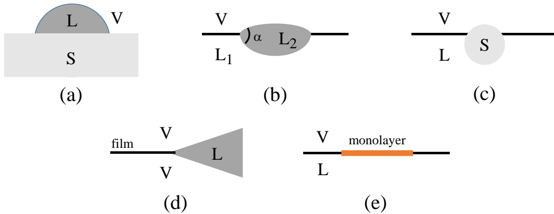
Fig. 1 Examples of three-phase contact lines, possessing line tension \tau , where three bulk phases meet: (a) liquid (L) droplet at a solid(S)-vapor(V) surface, (b) liquid droplet at a liquid-vapor surface, (c) solid particle at a liquid-vapor surface, and (d) thin film meeting a bulk liquid phase. Example of a two-dimensional discontinuity: (e) insoluble monolayer at a liquid-vapor surface.
