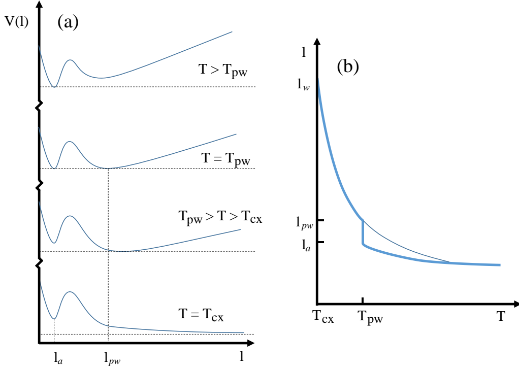
Fig. 6 (a) Variation in the surface potential V(l) in the vicinity of the pre-wetting ( T_{pw} ) and coexistence ( T_{cx} ) temperatures. (b) Corresponding variation in the pre-wetting thickness as a function of temperature. Heavy solid line: pre-wetting thickness at absolute minimum in V(l) for each temperature where a discontinuous jump in thickness is observed at T_{pw} with decreasing temperature. Light solid line: thicker pre-wetting film ( l_{pw} ) may become metastable with increasing temperature.
