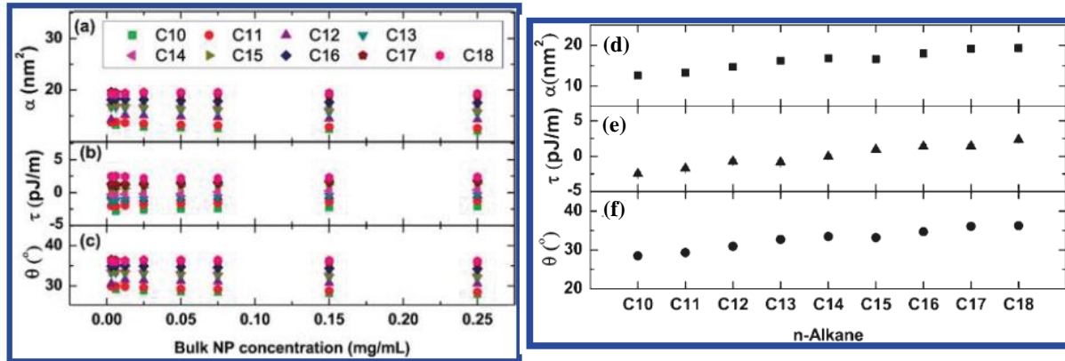
Fig. 16 (a) \alpha = \pi b^2 , (b) \tau , and (c) \theta versus bulk NP concentration for various n-alkane solvents deduced from Eqs. (35) – (38). Average values for (d) \alpha , (e) \tau , and (f) \theta for each n-alkane solvent. Reprinted (adapted) with permission from [31], © (2011) American Chemical Society.
