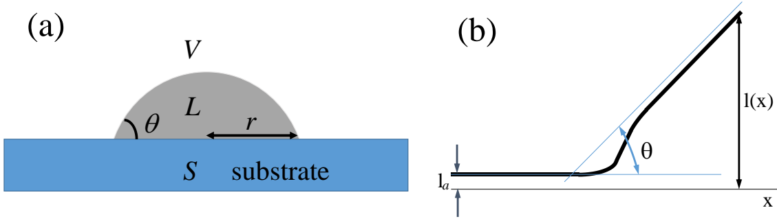
Fig. 2 (a) Liquid droplet (L) of lateral radius r and contact angle \theta at a substrate (S) – vapor (V) surface. (b) In the immediate vicinity of the three-phase SLV contact line, the liquid thickness l(x) varies with distance x along the substrate, from an adsorption thickness l_a on the vapor side ( x \ll 0 ), to a “liquid wedge” of contact angle \theta and thickness variation l(x) on the liquid side ( x \gg 0 ).
