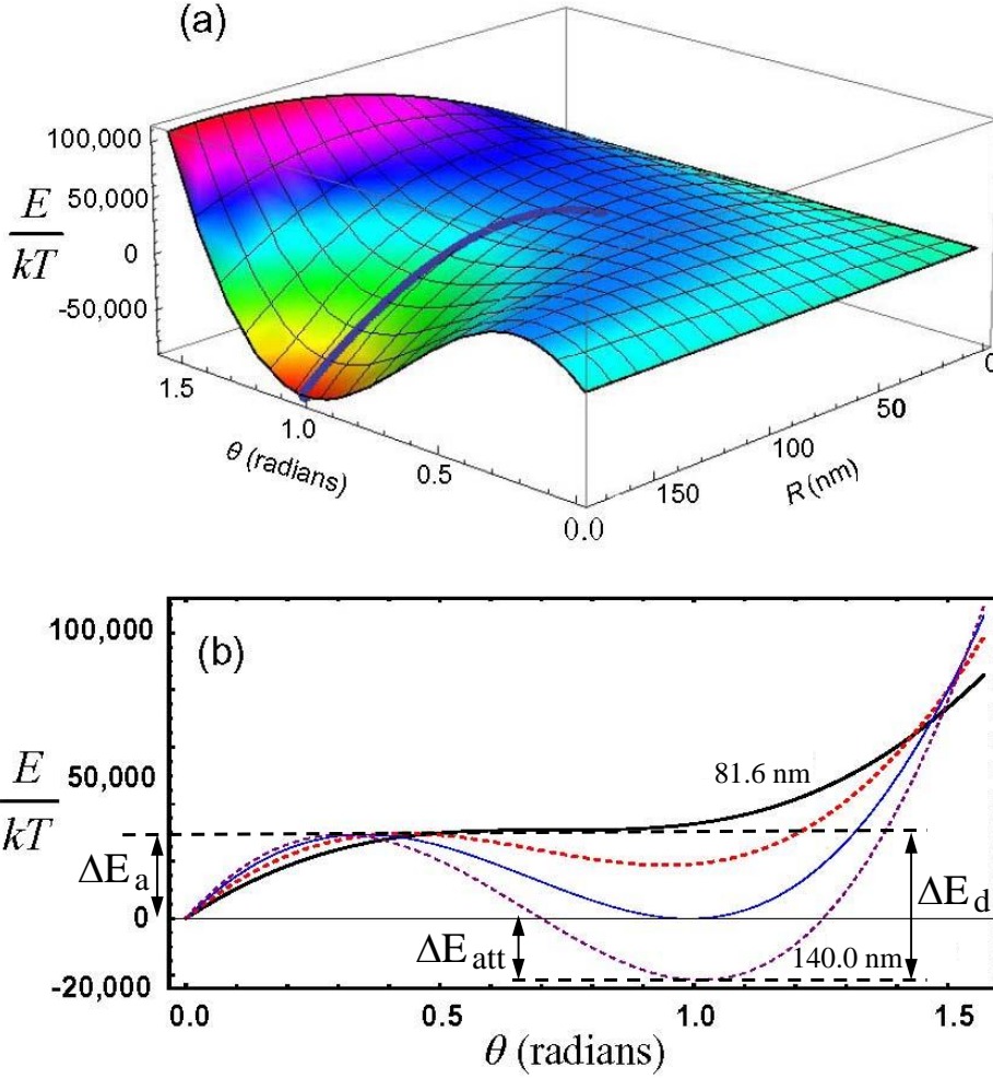
Fig. 13 (color online). (a) Energy E/kT Eq. (26) for \sigma_{LV} = 39.9 mN/m, \tau = 0.93 nN, and \theta_{\infty} = 64.8^{\circ} . Modified Young's equation Eq. (28), solid line. (b) Energy cross-sections at fixed R = 81.6, 105.0, 124.0 and 140.0 nm where R_{\min} = 81.6 nm Eq. (31), heavy solid line. For R = 140.0 nm, particle adsorption \Delta E_a , desorption \Delta E_d and attachment \Delta E_{att} energies are shown. Reprinted (adapted) with permission from [85], © (2012) American Physical Society.
