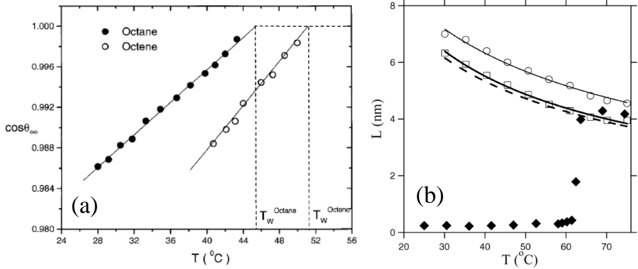
Fig. 4 (a) Variation of \cos\theta_\infty with temperature T for an octane and octene droplet on a hexadecyltrichlorosilane coated silicon wafer. At T_w \cos\theta_\infty = 1 . Reprinted (adapted) with permission from [9], © (1999) American Physical Society. (b) Thermal variation of wetting layer thickness on a hexadecyltrichlorosilane coated silicon wafer at a height H \sim 5 mm above n-hexane (circles), n-heptane (squares) and n-octane (diamonds) liquid. Reprinted (adapted) with permission from [81], © (2003) American Chemical Society.
