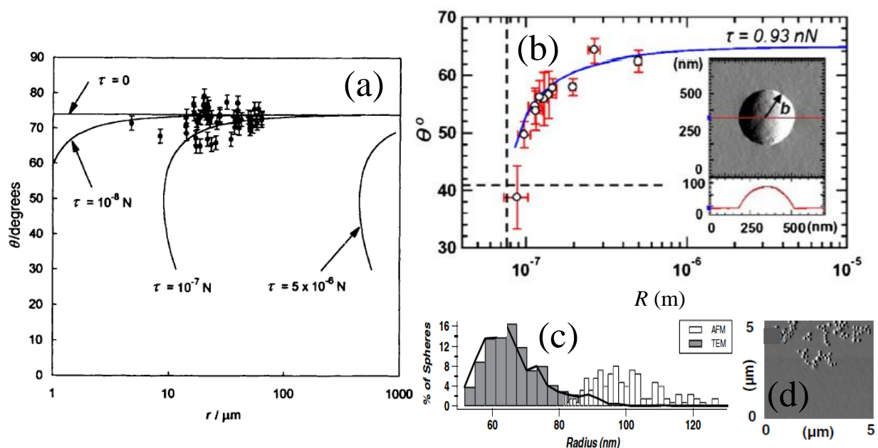
Fig. 14 (a) Optical microscopy contact angle \theta vs particle radius for fluorinated silica particles at dodecane-air surface. Reprinted (adapted) with permission from [86], © (1996) Royal Society of Chemistry. (b)-(d) Results for dodecyltrichlorosilane coated silica particles at PS-air surface. Reprinted (adapted) with permission from [85], © (2012) American Physical Society. (b) AFM contact angle \theta vs radius R . Vertical (horizontal) dashed line R_{\min} ( \theta_{\min} ). Inset: AFM phase image and cross-sectional height. (c) Polydisperse sample of average radius \sim 65\text{nm} measured via TEM (solid rectangles and solid line), surface distribution of this sample at PS-air surface measured via AFM (open rectangles). (d) AFM image of NPs at PS-air surface.
