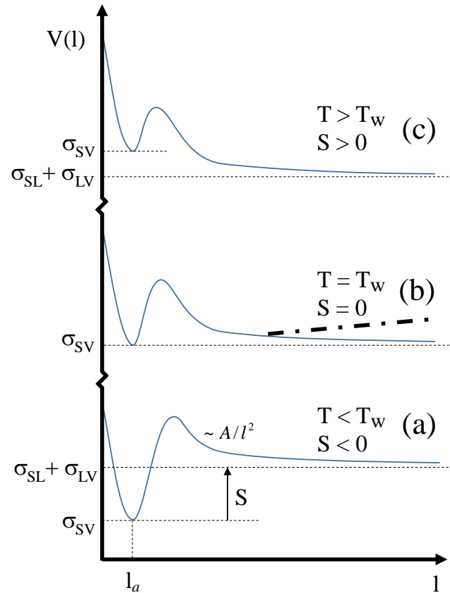
Fig. 5 Interaction potential V(l) as a function of liquid film thickness l on a solid substrate for Hamaker constant A > 0 for temperatures (a) below, (b) at, and (c) above the first-order wetting transition temperature T_w . This interaction potential is applicable for an n-octane droplet on an alkyl-silane coated silicon wafer, as described in the text. For T < T_w , in the vicinity of the three-phase SLV contact line, the film thickness varies as shown in Fig. 2b. The droplet is surrounded by an adsorbed film of thickness l_a and energy \sigma_{SV} on the vapor side of the 3-phase contact line. On the liquid side of the 3-phase contact line, l progressively thickens and approaches an energy of \sigma_{SL} + \sigma_{LV} . In (b) the dashed-dotted line indicates the change in shape due to the presence of an off-coexistence term \Delta\mu_l > 0 .
