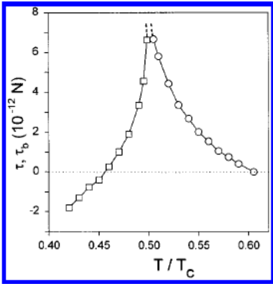
Fig. 9 Variation in line tension \tau with temperature for a pentane droplet on water on approaching (from below) a first-order wetting transition at T/T_c = 0.5 . The variation in the boundary tension \tau_b with temperature between an adsorbed film and a pre-wetting film is also shown in the one phase region ( T/T_c \geq 0.5 ). Reprinted (adapted) with permission from [84], © (1999) American Chemical Society.
