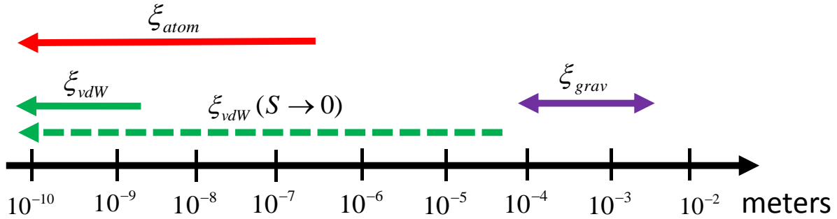
Fig. 27 Pictorial representation of the line tension length \xi (Eq. (2)) for the atomic \xi_{atom} , van der Waals \xi_{vdW} , and gravitational \xi_{grav} contributions to the line tension (solid arrows), far from a wetting transition. Near a wetting transition the line tension length defined in Eq. (6) must be used and, under these circumstances for example, the van der Waals line tension length \xi_{vdW}(S \rightarrow 0) may become very large (dashed line).
