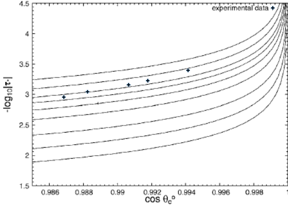
Fig. 24 Stability diagram for liquid droplets on a solid substrate where \tau^* is the reduced line tension (Eq. (64)) while the lines correspond to a residual stability index m_{rs} of 2 (lower curve), 5, 10, 20, 30, 40, 50, 70 and 100 (upper curve). The pluses are from experimental data for n-octane droplets on a silane-coated substrate [10]. Reprinted (adapted) with permission from [29], © (2006) American Physical Society.
