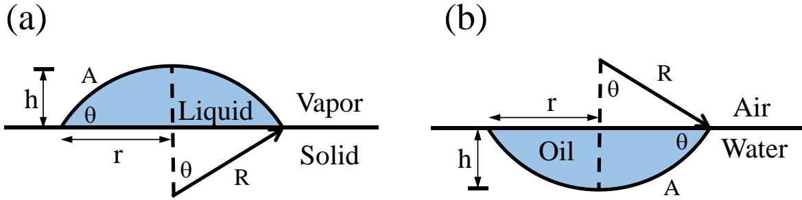
Fig. 17 (a) Liquid droplet on a flat solid substrate. Contact angle \theta , liquid-vapor radius of curvature R and area A , lateral radius r , and height h . (b) Oil droplet at the water-air surface, which is assumed flat.
