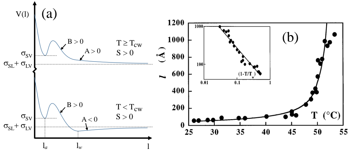
Fig. 7 (a) Interfacial potential V(l) for a second-order wetting transition where the Hamaker constant A changes sign with temperature. (b) Experimental measurements of thickness variation with temperature. Reprinted (adapted) with permission from [82], © (1996) American Physical Society.
