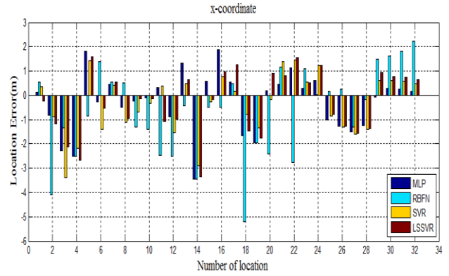
Fig. 10. Model localisation error in x-coordinate
