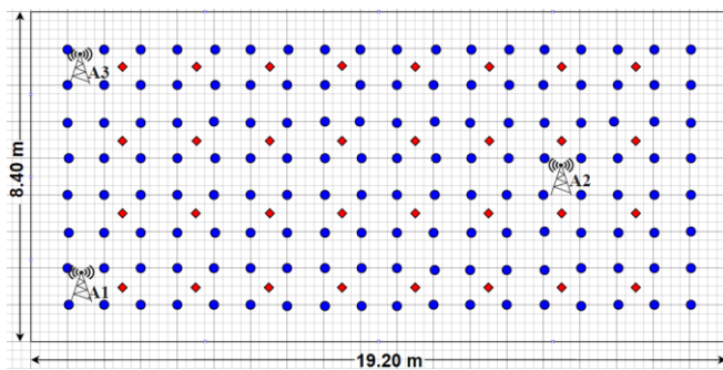
Fig. 6. Measurement grid for measurement campaign
