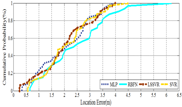
Fig. 13. CDF of model localization errors
