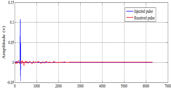
Fig. 8. Response of the receiver sensor for the injected PD pulse
