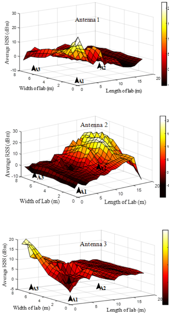
Fig. 9. Spatial variation of RSS for each antenna
