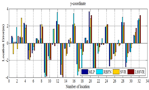
Fig. 11. Model localisation error in y-coordinate
