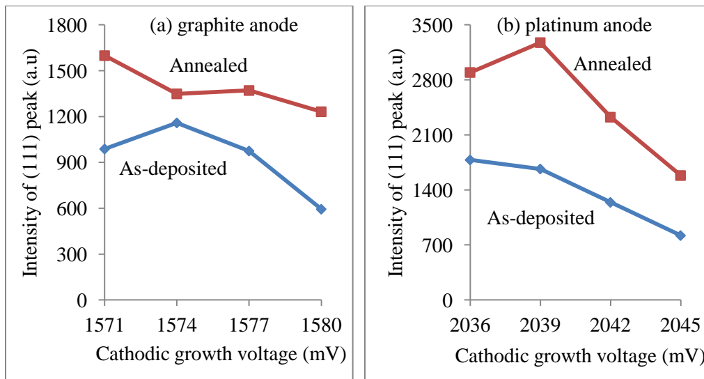
Figure 3: (111) XRD peak intensity vs. cathodic growth voltage for CdTe grown with (a) graphite anode and (b) platinum anode.
