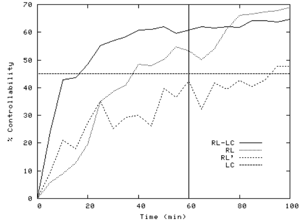
Fig. 5. Percentage of controllable cells over time for the 4 algorithms.
