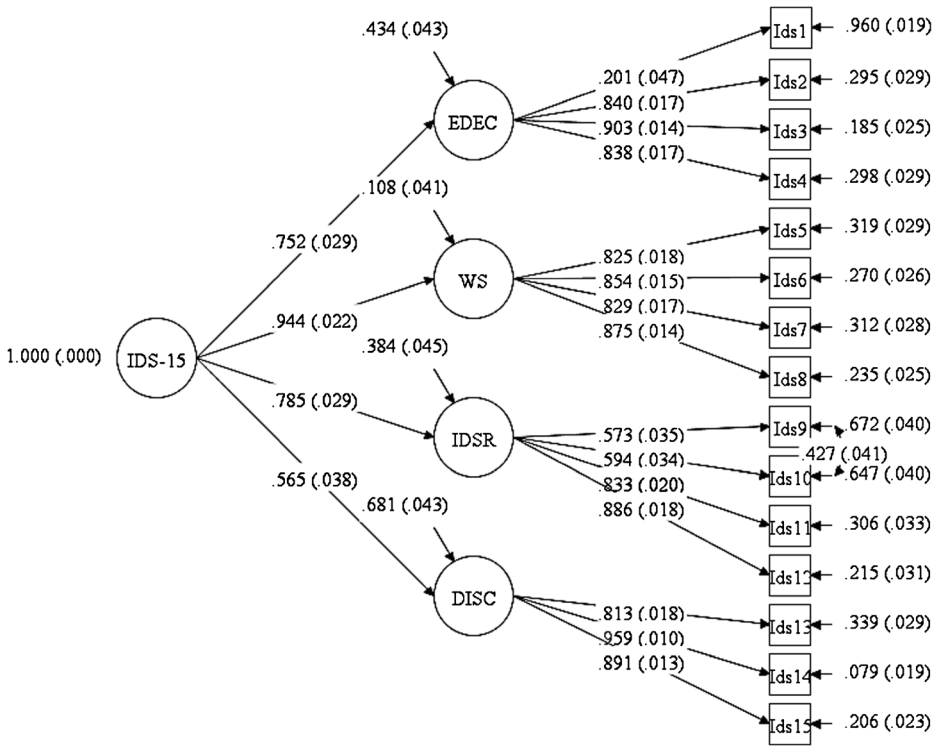
Fig. 1 Graphical representation of Model 3
