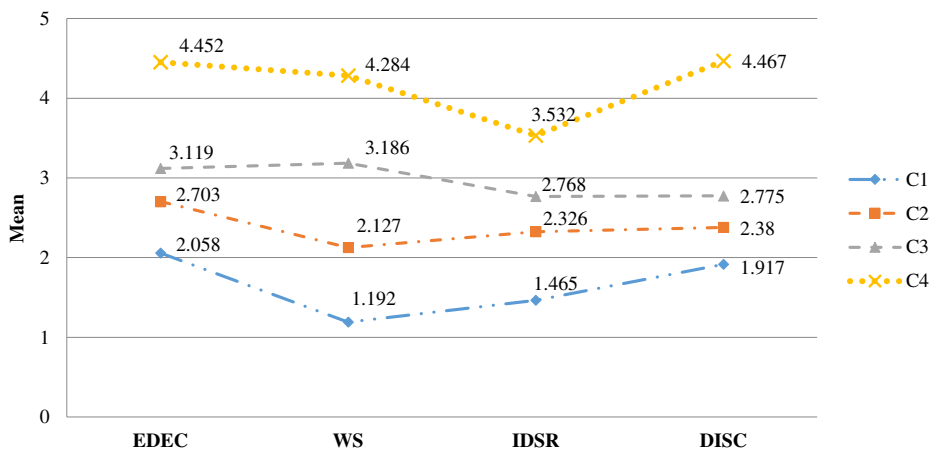
Fig. 2 The four-class solution obtained from the LPA. C1 low addiction risk, C2 medium addiction risk, C3 high addiction risk, and C4 critical addiction risk
