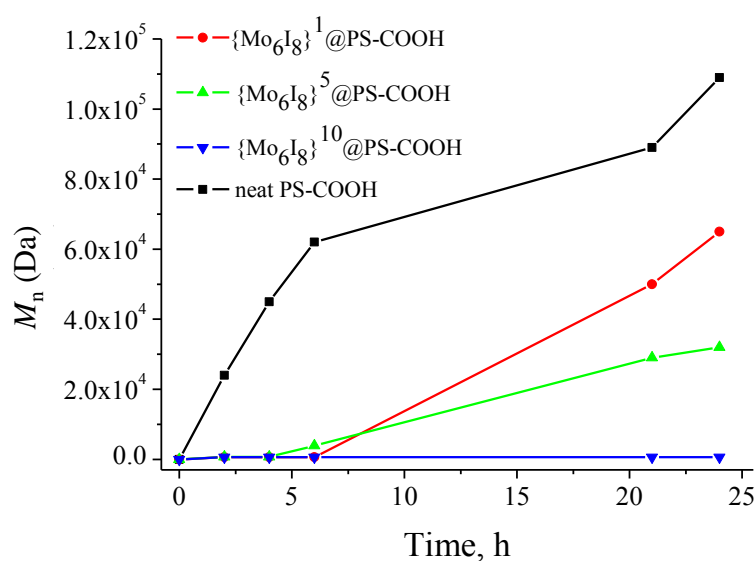
Figure 1. Molecular weight for neat PS-COOH and \{\text{Mo}_6\text{I}_8\}@PS\text{-COOH} materials with different cluster content
