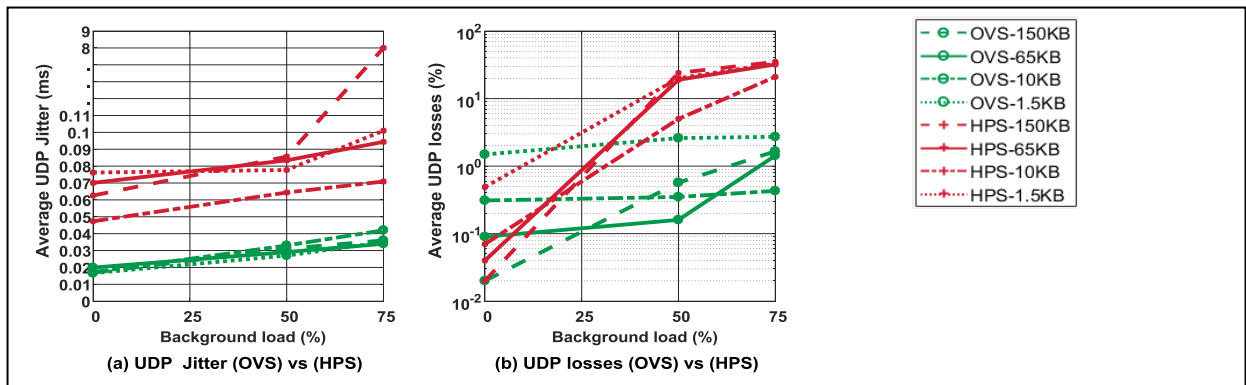
Fig.6. Jitter and losses packet rate measurement comparison between Mininet (OVS) and Physical testbed (HP Aruba) for UDP traffic using Iperf.
