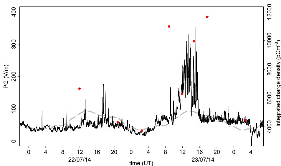
Fig. 6. Time series during the two days of the Alqueva IOP from 22nd to 24th July 2014. The black line denotes the PG, whilst the red dots show the calculated integrated space charge up to 5 km for each charge sensor balloon flight during the period (using Eq. (2)). The grey dash-dotted line shows the averaged diurnal variation in PG for fair weather days at the Alqueva site during the entire ALEX campaign. (For interpretation of the references to colour in this figure legend, the reader is referred to the web version of this article.)
