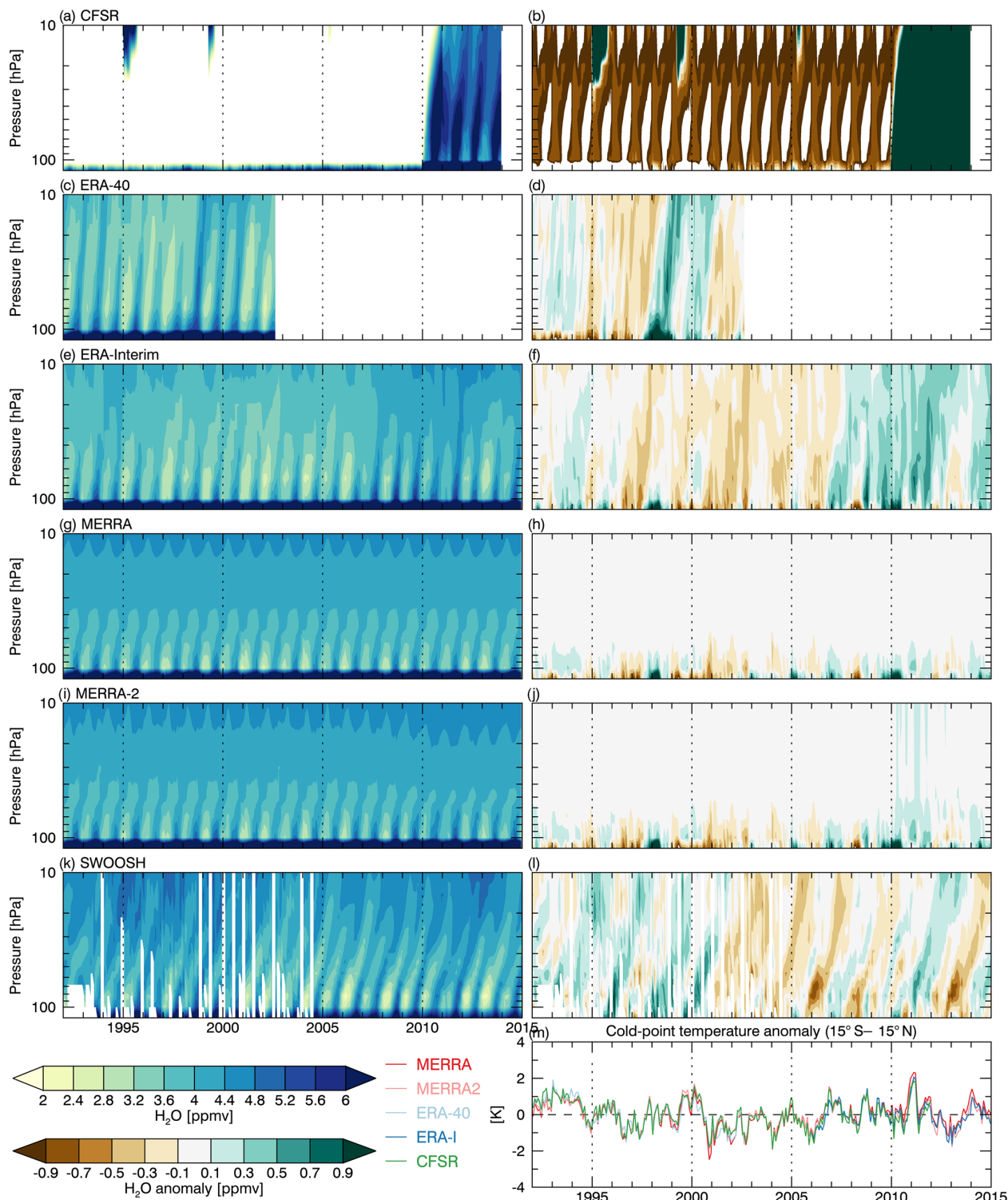
Figure 15. The tropical tape recorder signal as represented in reanalyses and the SWOOSH merged satellite product, defined as the height–time evolution of water vapor averaged over the 15°S–15°N tropical band. Both absolute values (a) and anomalies relative to the mean water vapor seasonal cycle at each level (b) are shown. Anomalies are computed separately for each data set. Monthly mean anomalies in tropical (15°S–15°N) cold-point tropopause temperatures calculated from 6 h data on the native vertical resolution of each reanalysis model are shown for context (m).
