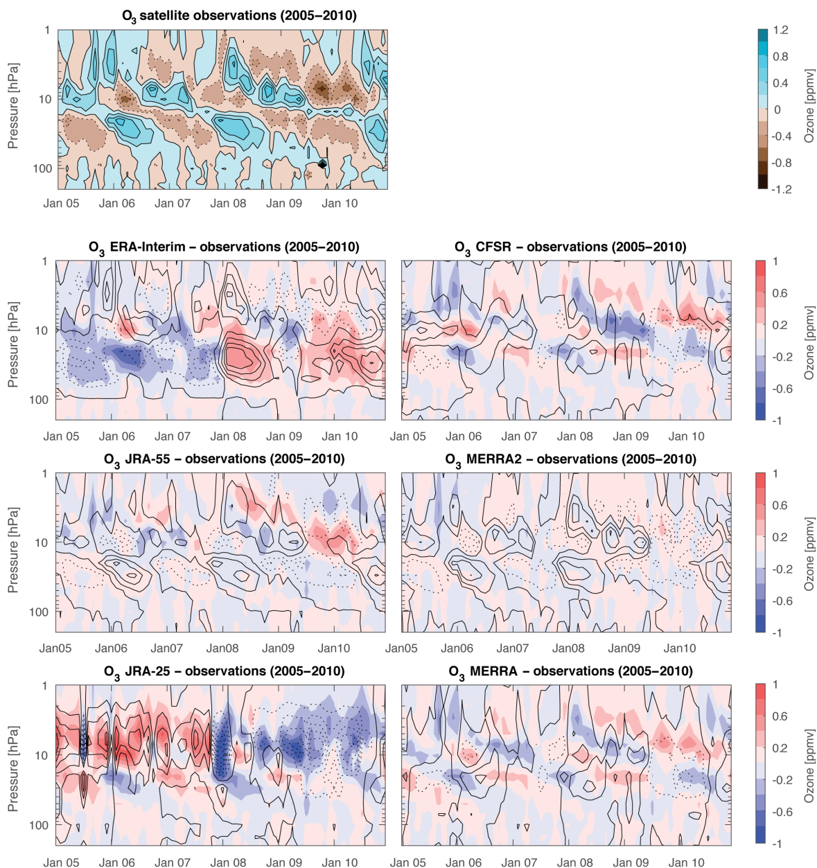
Figure 8. QBO ozone signal from the SPARC Data Initiative observations (upper left) during 2005–2010, defined as altitude–time cross sections of deseasonalized ozone anomalies averaged over the 10^\circ S– 10^\circ N tropical band. Observations are based on three satellite data sets. The other panels show the differences in QBO ozone signals between each reanalysis and the observations ( R_i - \text{MIM} , shaded contours), with the black line contours showing the QBO ozone signal generated by each corresponding reanalysis.
