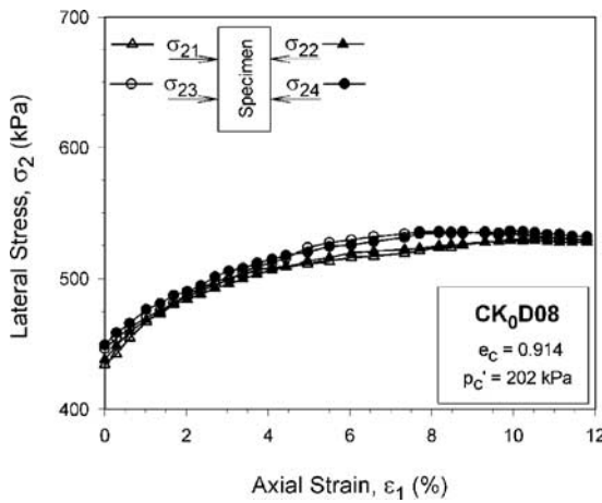
FIG. 2—The \sigma_2 versus \epsilon_1 curves obtained for a very loose specimen prepared by the moist tamping method.
