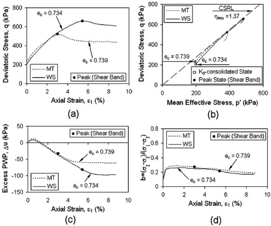
FIG. 7—Comparison of undrained ( de_v/de_1 = 0 ) strain path tests conducted on WS and MT specimens.
