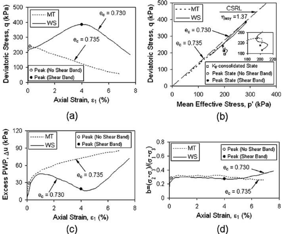
FIG. 8—Comparison of dilative ( de_v/de_1 = -0.2 ) strain path tests conducted on WS and MT specimens.
