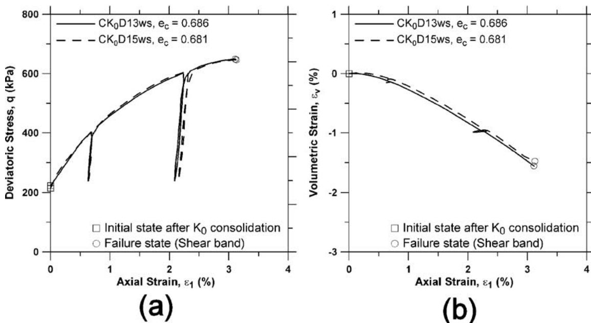
FIG. 1—Repeatability of drained tests under plane-strain condition: (a) stress-strain curves; (b) volumetric strain curves.
