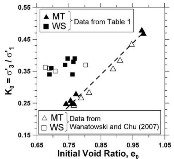
FIG. 4— K_0 versus e_0 plot determined for Changi sand.
