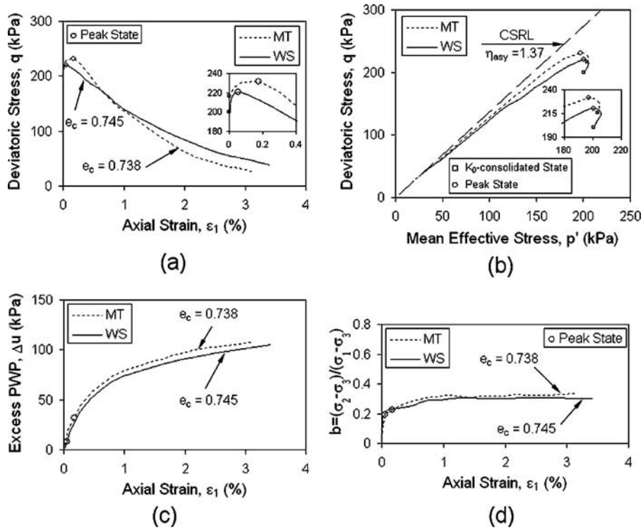
FIG. 9—Comparison of dilative ( \varepsilon_v/\varepsilon_1 = -0.6 ) strain path tests conducted on WS and MT specimens.
