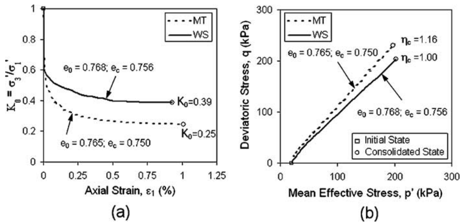
FIG. 5—Comparison of K_0 consolidation tests conducted on WS and MT specimens.
