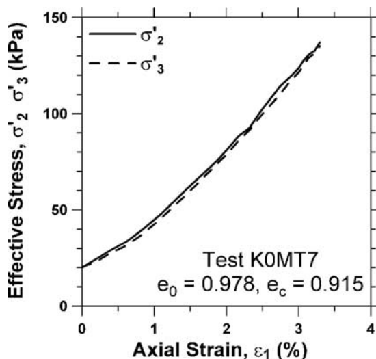
FIG. 3—The lateral stress response obtained from a K_0 consolidation test.
