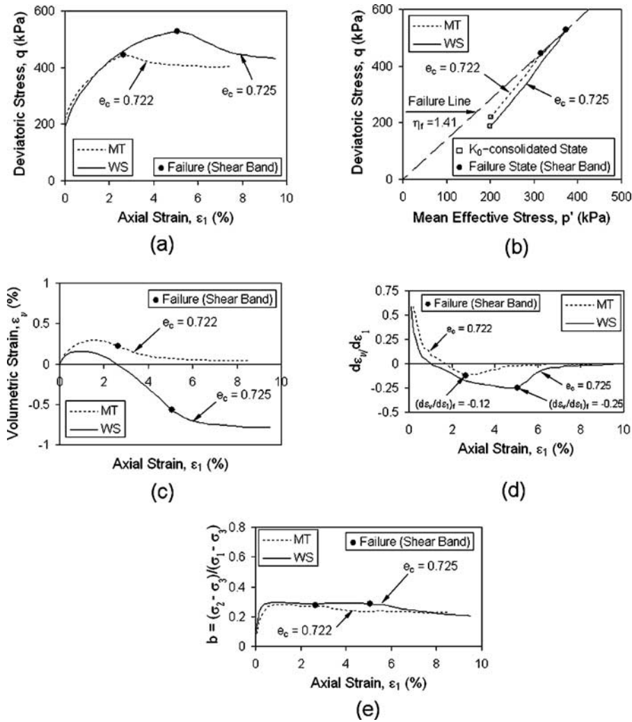
FIG. 6—Comparison of drained tests conducted on WS and MT specimens.
