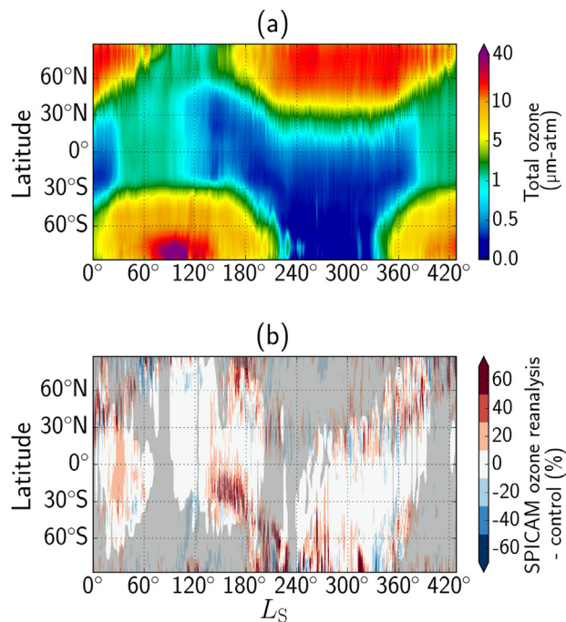
Fig. 3. Assimilated zonally averaged ozone column at 12 p.m. everywhere (top) and the percentage difference (SPICAM ozone reanalysis - control) between the SPICAM ozone reanalysis and control simulation (bottom) for MY 27 and start of MY 28. Shading indicates regions where there are no nearby SPICAM retrievals at the corresponding time and space.
