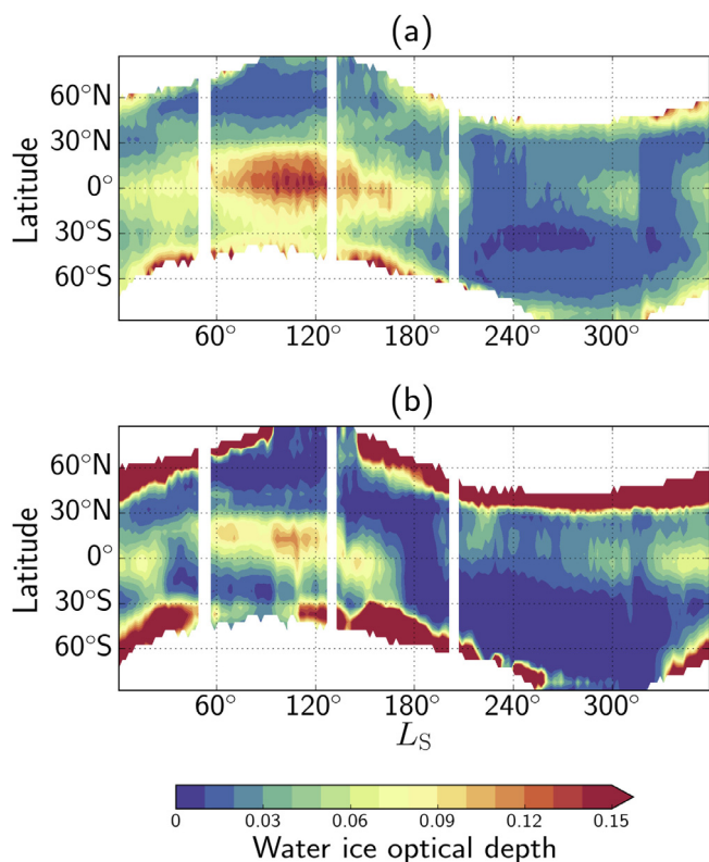
Fig. 6. (a) TES water ice optical depth retrievals at 825\text{ cm}^{-1} in MY 26 and (b) simulated zonal-averaged water ice optical depth at 825\text{ cm}^{-1} in the SPICAM ozone reanalysis at 2 p.m. local time covering MY 27. A mask has been applied to the model results to make the comparison clearer.
