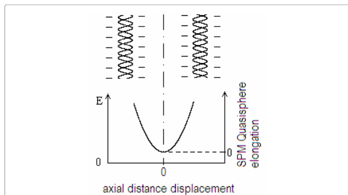
Figure 10: Electric field and SPM Quasisphere elongation between two parallel parts of DNA.
