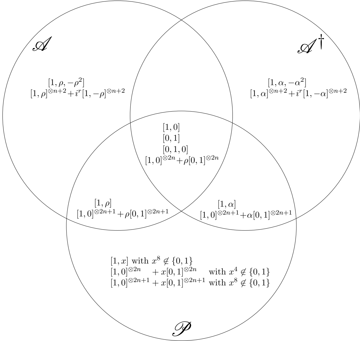
Figure 35: A Venn diagram of the #CSP 2 tractable sets \mathcal{A} , \mathcal{A}^\dagger , and \mathcal{P} . Note that \rho^4 = 1 , \alpha^4 = -1 , and n \geq 1 . Excluded are tensor products of unary signatures.
