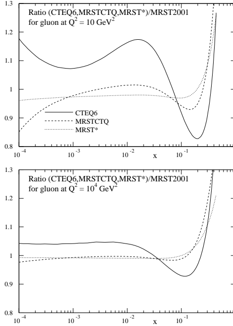
Fig. 2. Comparison of MRST2001 gluon distribution to the other distributions described in the text.
