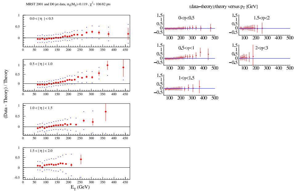
Fig. 1. Comparison of MRST fit to D0 jet data to CTEQ6 fit.
