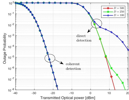
Fig. 9. Outage probability vs. transmitted optical power for thermal-noise-limited receivers with receiver temperature T^\circ = 295 K and local resistance R_L = 50 \Omega .
