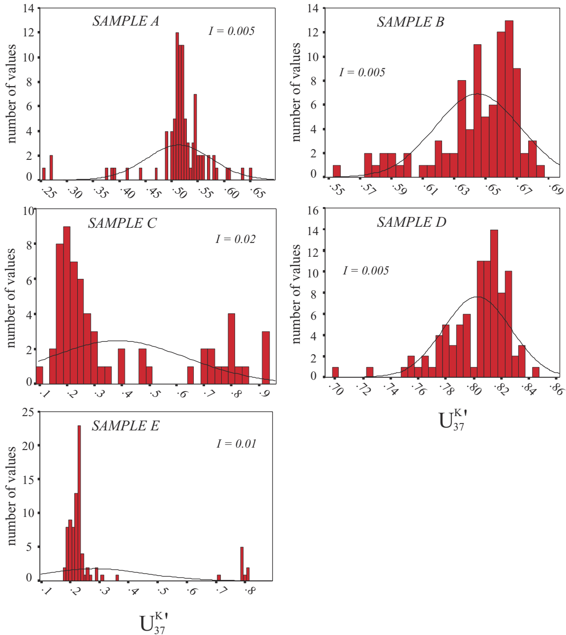
Figure 4. Histograms of all replicate measurements from each laboratory for the analysis of U_{37}^{K'} in the sediment test samples. The interval covered by each bar is indicated in each graph ( I ). The solid curve represents the normal distribution of the data.
