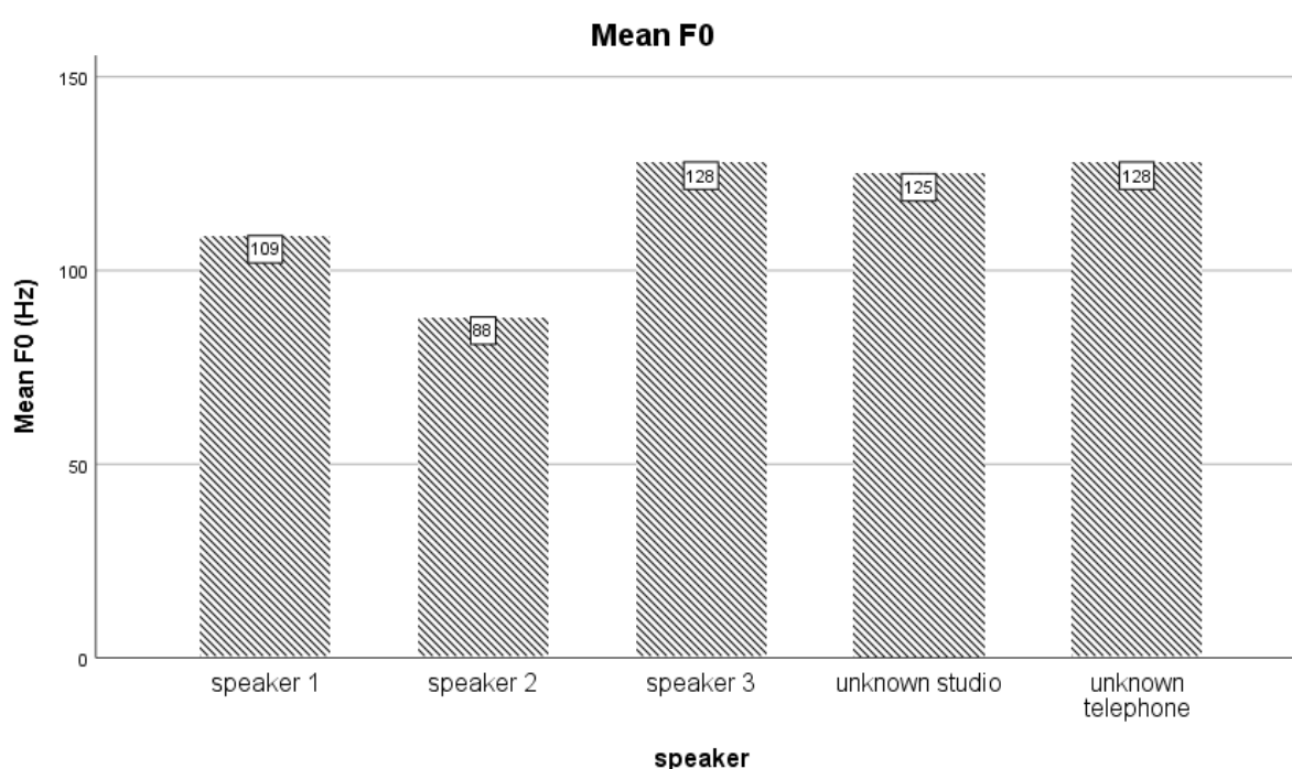
Figure 7. Bar graph of the mean F0 values for all the known speakers and both the unknown studio and the unknown telephone recording.
