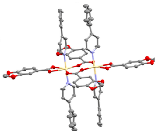
(4) [Cd(μ-Pip)(Pip)(4-Phpy) 2 ] 2
