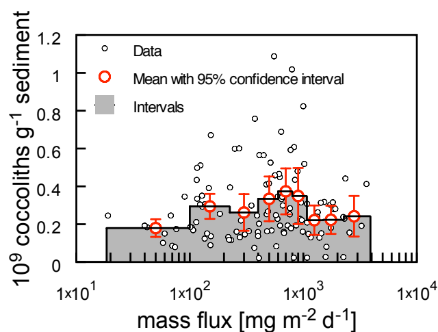
Figure 3. Emiliana huxleyi coccolith concentration in trap material versus total mass flux. Individual data points show an irregular scatter. Also the mean values within the mass flux intervals indicated by the grey bars show no increase with mass flux, indicating small influence of sediment transport and resuspension on coccolith concentration.
