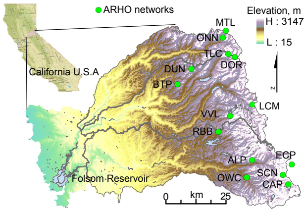
Fig. 1. The 14 low-power wireless networks deployed in the American River Hydrologic Observatory, near Sacramento, CA, USA. Each deployment site is identified by a 3-letter codename.
