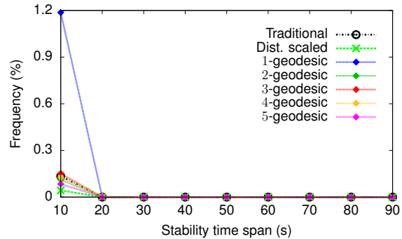
Fig. 12. In the highly dynamic scenario of the TAPASCologne vehicular network, the \rho -geodesic betweenness is the metric that changes less frequently the ranking of nodes. Of all nodes in the network, 1.2% remain in the same rank position for up to 10 seconds.
