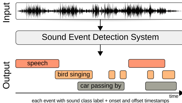
Figure 3: A schematic illustration of sound event detection in real-life audio addressed in Task 3.
