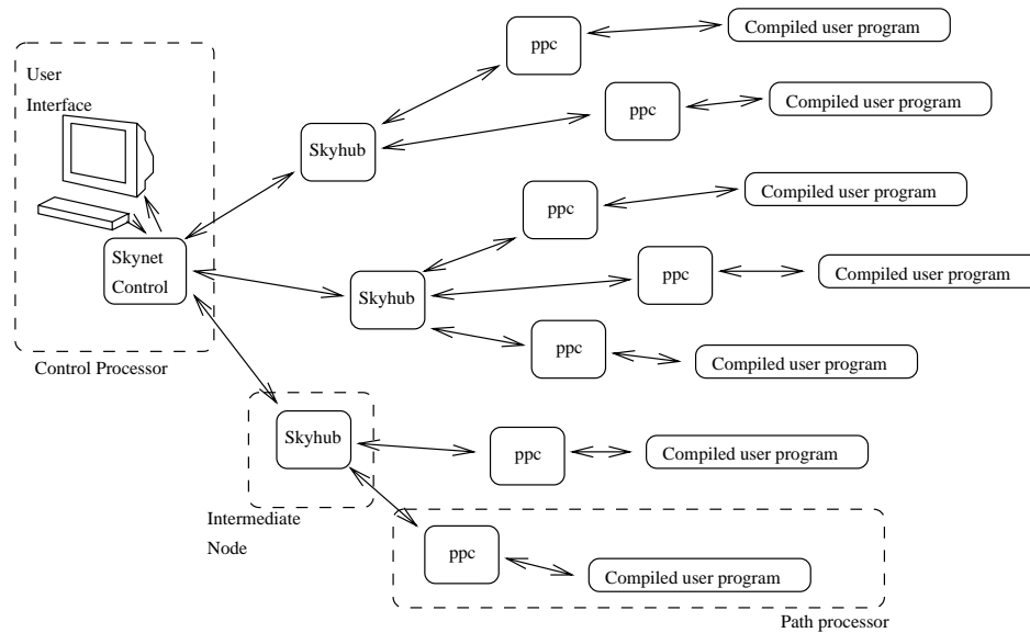
Figure A.1: System communications architecture
