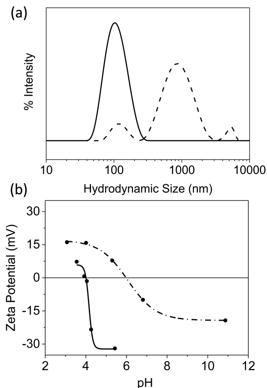
Figure 9. Effect of the citric acid (CA) coating on sample NF-4: (a) DLS measurements and (b) \zeta potential curves fitted to a Boltzmann sigmoidal function. Dashed line connects data points for the as-synthesized sample. The continuous line connects data points for citric acid coating.
