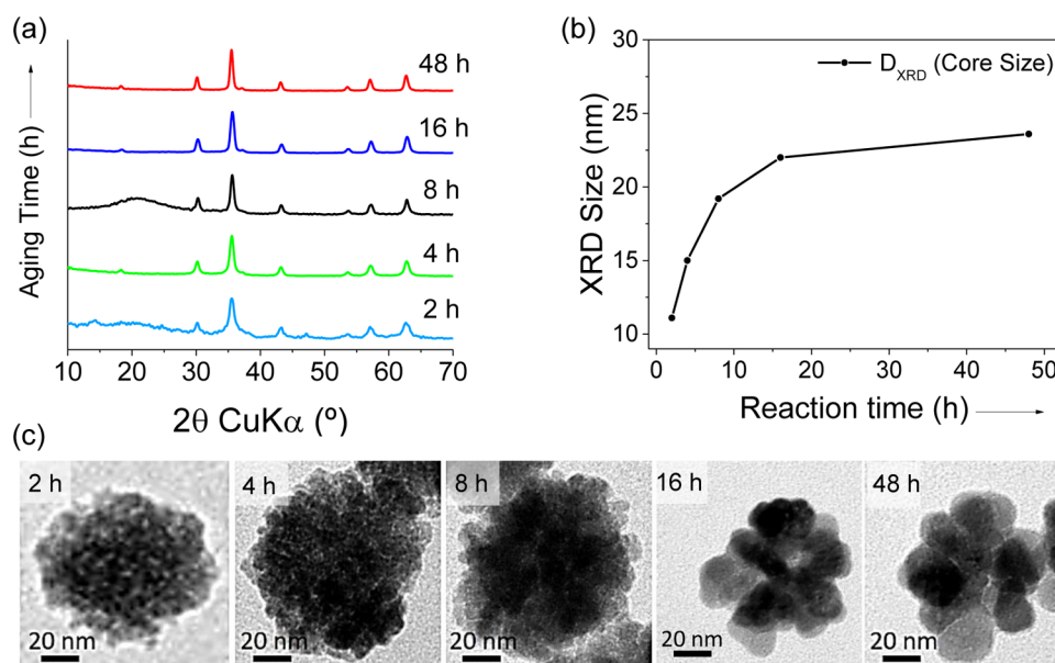
Figure 7. Structure of the NF along the formation at t = 2 –48 h: (a) XRD patterns, (b) core size calculated by Scherrer's equation. (c) representative TEM images of the growing cores.
