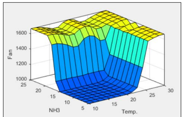
Figure 12. Temperature - NH 3
