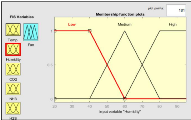
Figure 4. Membership of fuzzy set in humidity
