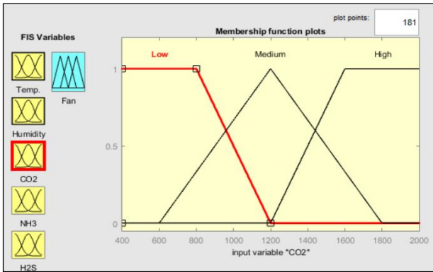
Figure 5. Membership of fuzzy set in CO 2
