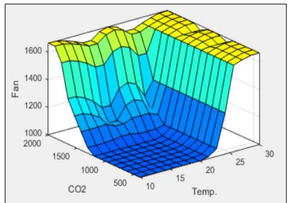
Figure 11. Temperature - CO 2
