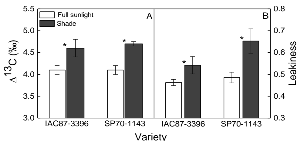
Fig. 6. Carbon isotope discrimination ( \Delta^{13}\text{C} , in A) and bundle sheath leakiness ( \phi , in B) in sugarcane varieties IAC87-3396 and SP70-1143 grown under full sunlight or shading for 48 days. Values are mean \pm SD ( n=4 ). * indicates significant difference ( P < 0.05 ) between light treatments in a given variety.
