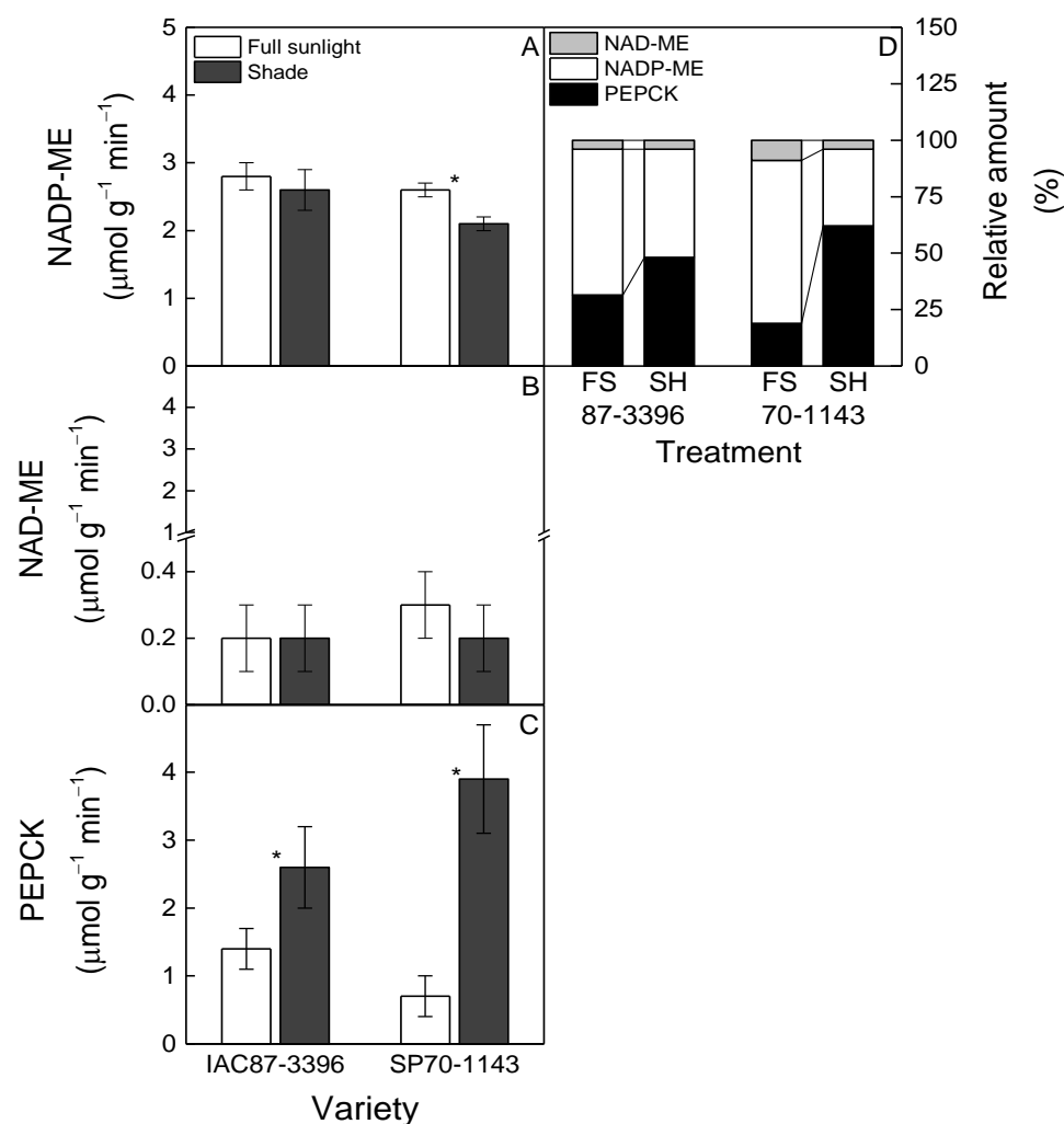
Fig. 4. Activity of NADP-ME (A), NAD-ME (B) and PEPCK (C), and their relative contribution of the overall decarboxylation (D) in sugarcane varieties IAC87-3396 and SP70-1143 grown under full sunlight (FS) or shading (SH) for 48 days. Values are mean \pm SD ( n=4 ). * indicates significant difference ( P < 0.05 ) between light treatments in a given variety.
