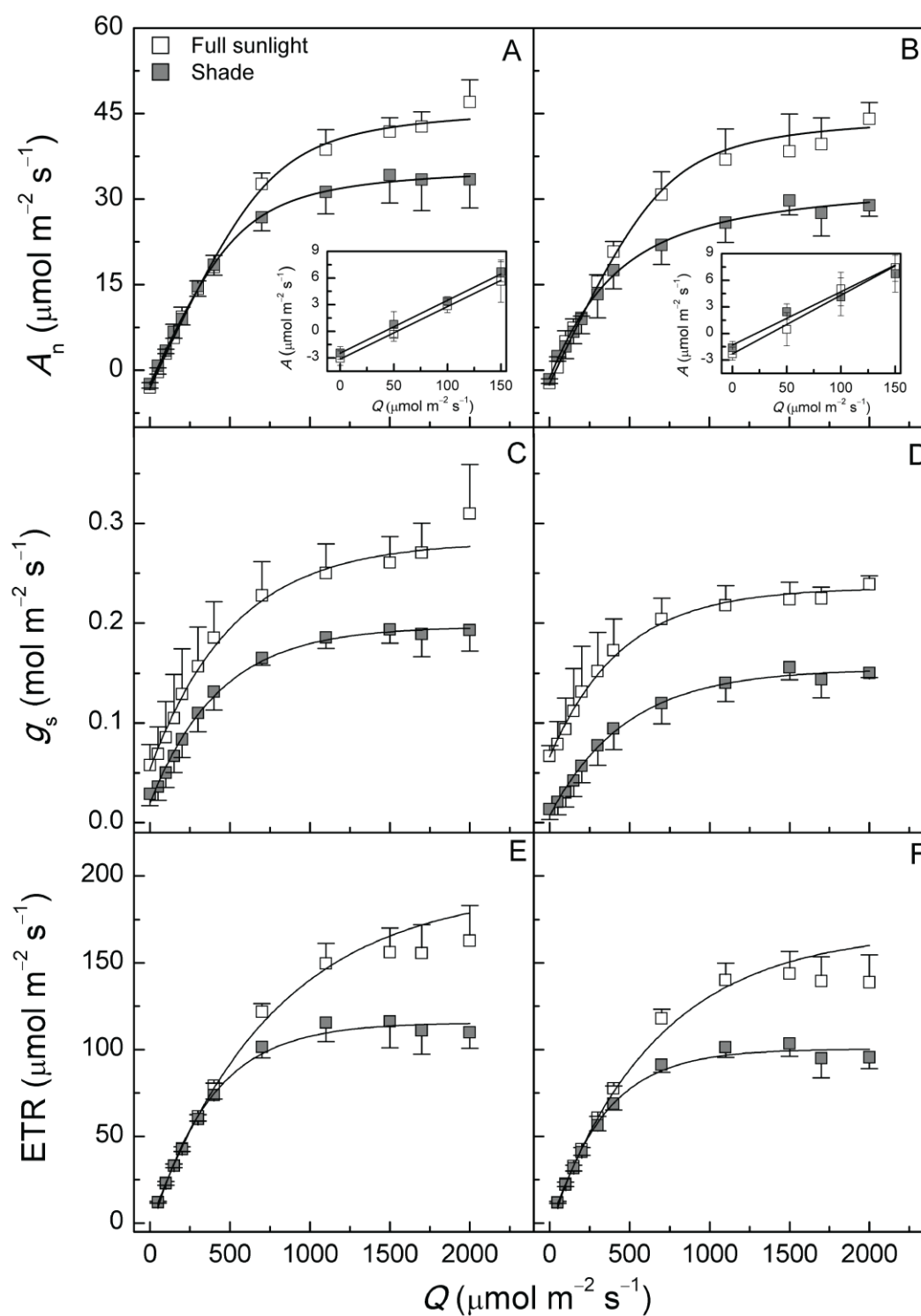
Fig. 1. Response of leaf \text{CO}_2 assimilation rate ( A_n in A and B), stomatal conductance ( g_s , in C and D) and apparent electron transport rate ( ETR , in E and F) to increasing photosynthetic active radiation ( Q ) in sugarcane varieties IAC87-3396 (A, C and E) and SP70-1143 (B, D and F) grown under full sunlight (open symbols) or shading (closed symbols) for 39-41 days. Curves in A and B were fitted according to Marshall and Biscoe (1980). Values are mean \pm SD ( n=4 ).
