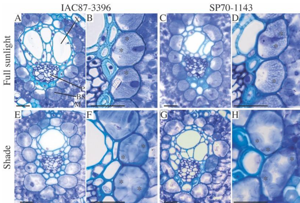
Fig. 5. Leaf cross sections of sugarcane varieties IAC87-3396 (A, B, E and F) and SP70-1143 (C, D, G and H) grown under full sunlight (A-D) or shading (E-H) for 48 days. General view of the vascular bundle (A, C, E, G) and detail of the bundle sheath cells (B, D, F, H) showing the chloroplast distribution: centrifugal (A-D) or evenly (E-H) positions. BS, bundle sheath; M, mesophyll, P, phloem; X, xylem; *, chloroplasts. Scale bar: 25 \mu\text{m} .
