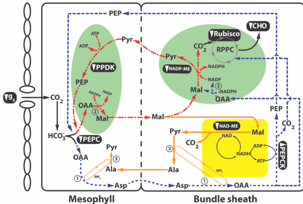
Fig. 7. Proposed model of sugarcane decarboxylation flexibility under shading. Reactions via NADP-ME (dash-point-dash lines), via NAD-ME (continuous lines) and via PEPCK (dashed lines). As it was not possible to discern in which extent in vitro NAD-ME activity detected in this study is from the photosynthetic metabolism, providing \text{CO}_2 for the Calvin cycle, or from the respiratory pathway, \text{CO}_2 released via this decarboxylation pathway are not directed to RPPC. Abbreviations: Ala, alanine; Asp, aspartate; CHO, carbohydrate; RPPC, reductive pentose phosphate cycle; g_s , stomatal conductance; Mal, malate; OAA, oxaloacetate; PEP, phosphoenolpyruvate; Pyr, pyruvate. (1), (2) and (3) represent the enzymes aspartate aminotransferase, NADPH-malate dehydrogenase, and alanine aminotransferase, respectively. Chloroplasts are in green (ellipsis) and mitochondria in yellow (square). Variables outlined in black were evaluated herein and arrows represent the response to shading: increase (▲) or decrease (▼). Adapted from Furbank (2011).
