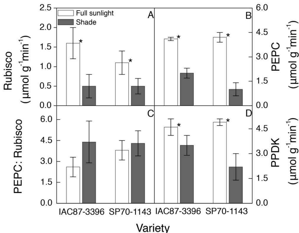
Fig. 3. Activity of Rubisco (A) and PEPC (B), PEPC:Rubisco ratio (C) and PPDK activity (D) in sugarcane varieties IAC87-3396 and SP70-1143 grown under full sunlight or shading for 48 days. Values are mean \pm SD ( n=4 ). * indicates significant difference ( P < 0.05 ) between light treatments in a given variety.
