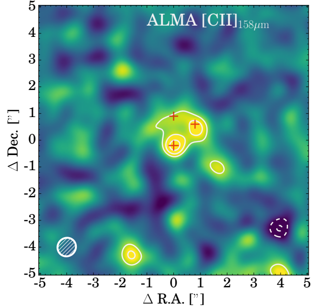
Figure 1. ALMA [CII] narrow-band image of CR7, collapsed for frequencies with -614 to +96 \text{ km s}^{-1} with respect to the \text{Ly}\alpha reference frame ( z = 6.604 ). The image ( 54 \times 54 \text{ kpc} ) is centred on the peak of \text{Ly}\alpha position and the ALMA astrometry is shifted by 0.25'' to the west to align it with HST imaging as described in §3.2. Contours are shown at the 3, 4, 5 \sigma significance levels (with 1\sigma = 0.016 \text{ Jy beam}^{-1} \text{ km s}^{-1} ). The beam size is shown in the bottom left corner and has FWHM 0.82'' \times 0.77'' . The red crosses mark the positions of the UV clumps of CR7. [CII] is clearly detected in CR7, indicating the presence of carbon.
