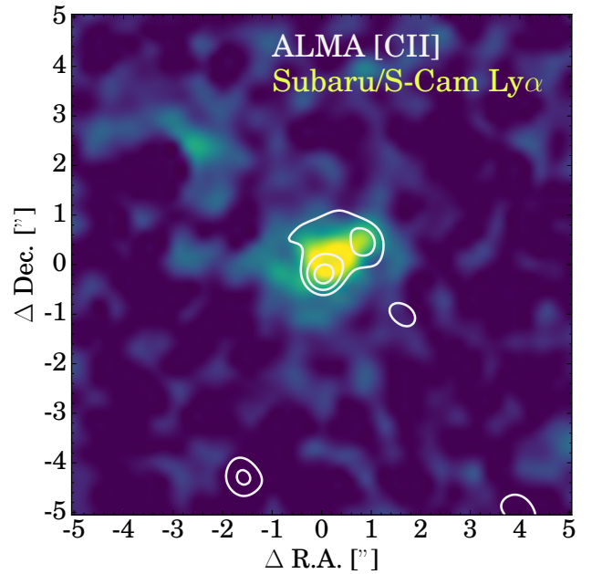
Figure 11. Rest-frame Ly \alpha image (from Subaru/S-Cam NB921 and z' band imaging) of CR7, overlaid with ALMA [CII] contours, with a scale of 54 \times 54 kpc. The Ly \alpha surface brightness is closely related to the [CII] surface brightness. At clump A, Ly \alpha is redshifted with respect to [CII] by 127 \pm 27 \text{ km s}^{-1} .
