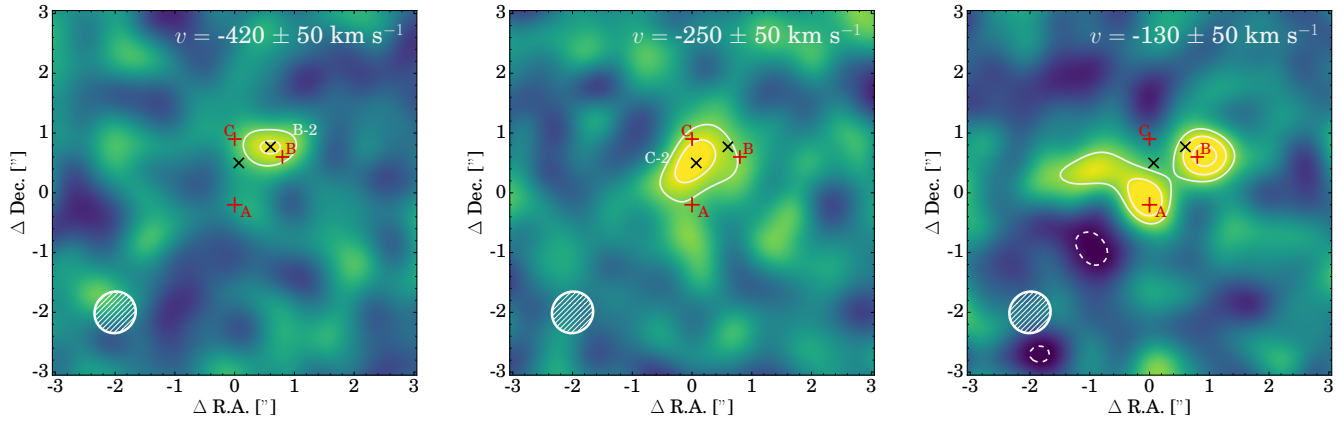
Figure 4. [CII] map in three velocity channels of 100 \text{ km s}^{-1} , zoomed in on CR7 (with a scale of 16 \times 16 \text{ kpc} ) and with velocities with respect to the \text{Ly}\alpha redshift of z = 6.604 . Contours mark the 3, 4, 5 \sigma levels, with sensitivities \sigma \approx 5 - 6 \text{ mJy beam}^{-1} \text{ km s}^{-1} . Red crosses mark the positions of the UV clumps, while black crosses mark the positions of additional [CII] components B-2 and C-2. The most luminous [CII] components coincide with UV clumps A and B and have a similar peak velocity. Fainter [CII] flux is detected at > 4\sigma in between clumps A, B and C offset by -120 \text{ km s}^{-1} , and close to clump B (at -290 \text{ km s}^{-1} ).
