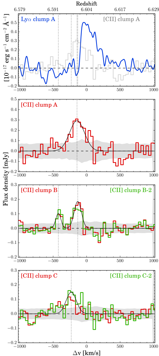
Figure 6. Flux densities of Ly \alpha (from X-SHOOTER, centered at clump A) and [CII] at the HST positions of clumps A, B and C as a function of velocity with respect to the Ly \alpha peak velocity at z = 6.604 . We also measure [CII] line-profiles at the positions B-2 and C-2 (shown in green), based on [CII] detections, see Fig. 4. Gaussian fits are shown in black, and we highlight the central velocities with vertical dotted lines. Errors have been estimated for each velocity-slice and aperture as described in §3.3.
