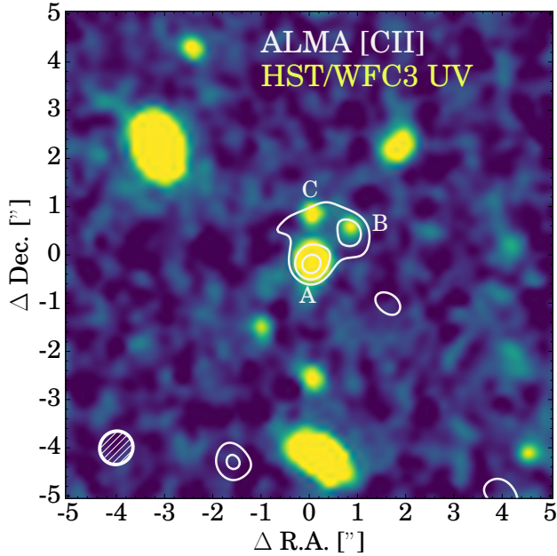
Figure 5. Rest-frame UV image (from HST /WFC3 F110W imaging) of CR7, overlaid with ALMA [CII] 3, 4, 5 \sigma contours at a scale of 54 \times 54 kpc. The names of the three UV clumps are annotated in HST imaging. Relatively compact components of [CII] emission are detected around clumps A and B, while there is diffuse [CII] emission covering clump C, although at lower significance.
