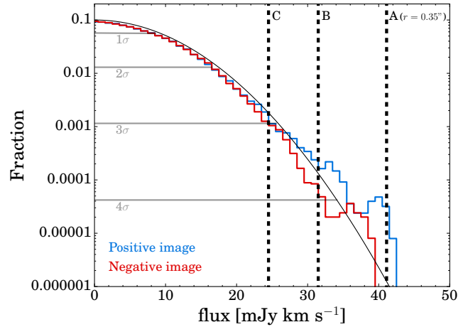
Figure 3. Histogram of the integrated [CII] fluxes measured over circular, beam-sized scales at random positions in the collapsed cube (with velocities from -614 to +96 km s ^{-1} with respect to Ly \alpha ). The blue histogram shows positive fluxes, while the red histogram shows negative fluxes. We indicate the [CII] flux measured at the positions of HST clumps A, B and C with vertical lines. These correspond to \approx 5, 4, 3\sigma detections, respectively. The grey curve shows the expected noise properties if the noise is gaussian with a 1\sigma dispersion. Note that our final measurement of clump A uses a larger aperture (with radius 0.55'' ), resulting in a similar significance but higher flux. Also note that the detections are at slightly higher significance in narrower-velocity slices optimised for each clumps specifically.
