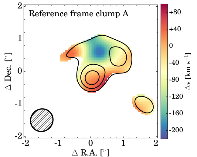
Figure 7. [CII] velocity map (at a 22 \times 22 kpc scale) in the rest-frame of clump A, based on the first moment map collapsed for frequencies with -614 to +96 \text{km s}^{-1} with respect to the Ly \alpha redshift (see Fig. 1 for the corresponding [CII] flux map). Contours show the 3, 4 and 5 \sigma threshold and velocity maps are shown for > 3\sigma detections. The map is driven by the the strongly blue-shifted component C-2.
