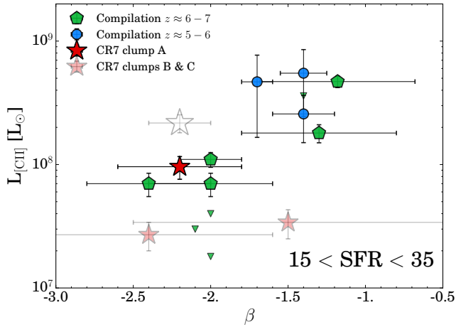
Figure 10. The relation between [CII] luminosity and UV slope, \beta , for galaxies with SFRs between 15 - 35 M_{\odot} \text{ yr}^{-1} . Galaxies with redder colours are typically more evolved (older, higher metallicity), and consequently have higher [CII] luminosities. For reference, we show the measurements of clumps B, C and the total of CR7 in fainter colours.
