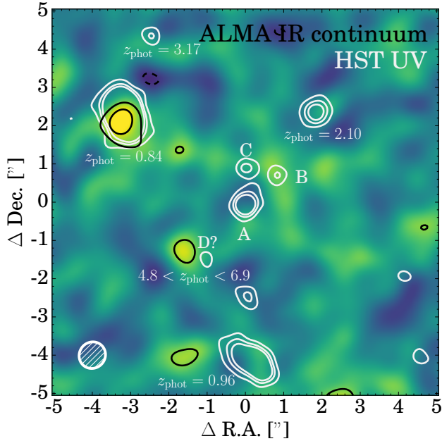
Figure 8. IR continuum map at 230-250 GHz centered on the position of CR7. The black contours show the 2, 3 \sigma level, where 1\sigma = 7\mu\text{Jy beam}^{-1} . We also show HST rest-frame UV (F814W+F110W+F160W) contours to highlight the positions of known (foreground) sources. Sources are annotated with their photometric redshifts estimated by Laigle et al. (2016). No dust continuum is detected at CR7, although a \approx 2\sigma signal is detected around potential clump D. Dust continuum is also clearly detected in a foreground source at z = 0.84 .
