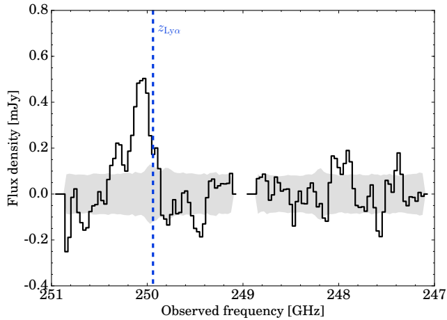
Figure 2. Integrated spectrum over the area within the 3\sigma [CII] contours in Fig. 1, in two observed spectral windows. The grey shaded region indicates the 1\sigma error estimated using apertures with the same geometry as the 3\sigma contour area, as a function of frequency. The blue dashed line indicates where [CII] would be detected at z = 6.604 , the Ly \alpha redshift of CR7. Ly \alpha is redshifted by \approx -170 km s ^{-1} with respect to the systemic [CII] redshift.
