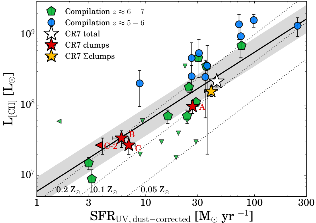
Figure 9. Dust corrected SFR(UV) versus [CII] luminosity for a compilation of galaxies at z \sim 6 (blue circles; Capak et al. 2015; Willott et al. 2015) and z \sim 7 (green pentagons; Kanekar et al. 2013; Ouchi et al. 2013; Ota et al. 2014; Maiolino et al. 2015; Schaerer et al. 2015; Knudsen et al. 2016; Pentericci et al. 2016; Bradač et al. 2017; Knudsen et al. 2017; Smit et al. 2017). We show the individual UV components of CR7 with red stars, and the sum of these component as an orange star. The integrated measurement over the full [CII] emitting region around CR7 is shown with an open star. The black line shows the relation for local star-forming galaxies measured by De Looze et al. (2014), where the grey region shows the observed dispersion. The dotted lines are model-predictions from Vallini et al. (2015) on how the [CII] luminosity varies with metallicity. We find that the clumps in CR7 are within the scatter from the local relation. These measurements indicate metallicities 0.1 < Z/Z_{\odot} < 0.2 . Note that we have corrected published SFRs (including those from the local relation) to the Salpeter IMF.
