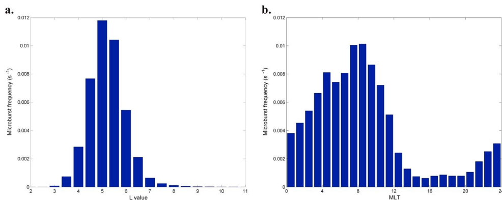
Figure 4. (a) The L distribution and (b) the MLT distribution of the frequency of occurrence of relativistic microbursts, corrected for satellite sampling bias.
