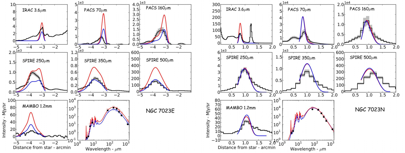
Fig. 13. The comparison of the modelled (blue and red curves) to observed data (black curves) at different wavelengths is shown. The intensity is plotted versus the angular distance from the star in arcmin. The grey zones stand for the photometric uncertainties and correspond to 5% for IRAC, 20% for PACS, and 15% for SPIRE. The blue curves show the results of our model and the red curves of the model from Compiegne et al. (2011) in comparison.
