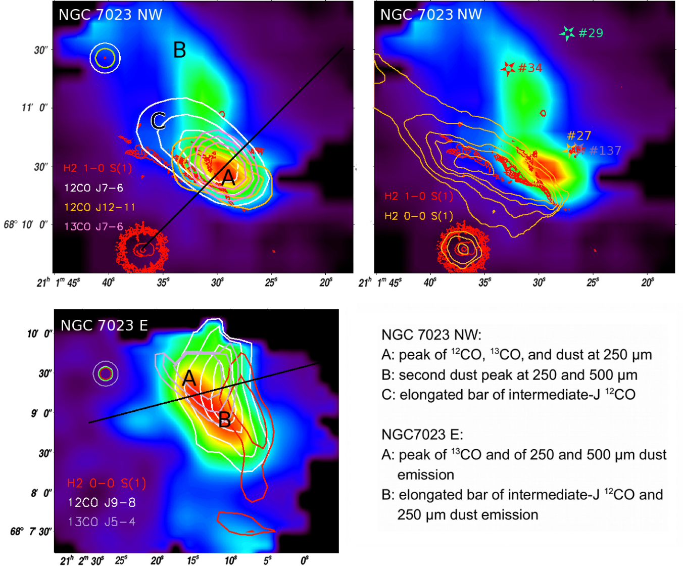
Fig. 6. Top left: FTS map at 250\ \mu\text{m} of the PDR NGC 7023 NW with contours of ^{12}\text{CO}\ J=7-6 (white), (maximum at 1.5 \times 10^{-5}\ \text{erg cm}^{-2}\text{s}^{-1}\text{sr}^{-1} with contour lines at 0.4, 0.6, 0.8 times the maximum), ^{12}\text{CO}\ J=12-11 (orange) (maximum at 4.0 \times 10^{-5}\ \text{erg cm}^{-2}\text{s}^{-1}\text{sr}^{-1} with contour lines at 0.2, 0.4, 0.6 times the maximum), and ^{13}\text{CO}\ J=7-6 (pink) (maximum at 3.2 \times 10^{-6}\ \text{erg cm}^{-2}\text{s}^{-1}\text{sr}^{-1} with contour lines at 0.4, 0.6, 0.8 times the maximum) and \text{H}_2\ 1-0\ \text{S}(1) (red) from Lemaire et al. (1996) (maximum at 3.7 \times 10^{-4}\ \text{erg cm}^{-2}\text{s}^{-1}\text{sr}^{-1} with contours at 0.27, 0.41, 0.55, 0.69 times the maximum). Top right: FTS map at 250\ \mu\text{m} of the PDR NGC 7023 NW with contours of \text{H}_2\ 0-0\ \text{S}(1) (orange) from Spitzer observations (maximum at 1.9 \times 10^{-4}\ \text{erg cm}^{-2}\text{s}^{-1}\text{sr}^{-1} with contour lines at 0.26, 0.36, 0.52, 0.62, 0.83 times the maximum) and \text{H}_2\ 1-0\ \text{S}(1) (red) (maximum at 3.7 \times 10^{-4}\ \text{erg cm}^{-2}\text{s}^{-1}\text{sr}^{-1} with contours at 0.27, 0.41, 0.55, 0.69 times the maximum). Bottom: FTS map of the PDR NGC 7023 E, 250\ \mu\text{m} map with contours of ^{12}\text{CO}\ J=9-8 (white) (maximum at 3.2 \times 10^{-6}\ \text{erg cm}^{-2}\text{s}^{-1}\text{sr}^{-1} with contour lines at 0.4, 0.6, 0.8 times the maximum), ^{13}\text{CO}\ J=5-4 (violet) (maximum at 5.6 \times 10^{-7}\ \text{erg cm}^{-2}\text{s}^{-1}\text{sr}^{-1} with contour lines at 0.7, 0.8, 0.9 times the maximum) and \text{H}_2\ 0-0\ \text{S}(1) (red) from Spitzer observations (maximum at 1.3 \times 10^{-4}\ \text{erg cm}^{-2}\text{s}^{-1}\text{sr}^{-1} with contour lines at 0.45, 0.66 times the maximum). Note that the FTS map at long wavelengths (SLW) is slightly smaller than the shown map, so that the ^{13}\text{CO}\ J=5-4 contour lines are cut off in the north. The letters A, B, and C indicate positions of interest as explained. We include the detected YSOs by Kirk et al. (2009) as stars in the top right figure. The FWHM of the beam for the different CO and the beam size for \text{H}_2 lines are presented. Maps: 12.2'' (green). NGC 7023 NW: 11.6'' for ^{12}\text{CO}\ J=12-11 (orange), 18.6'' for ^{12}\text{CO}\ J=7-6 (white), 18.7'' for ^{13}\text{CO}\ J=7-6 (white) and 1'' for \text{H}_2\ 1-0\ \text{S}(1) (red). NGC 7023 E: 13.0'' for ^{12}\text{CO}\ J=9-8 (white), 22.7'' for ^{13}\text{CO}\ J=5-4 (violet) and 11'' for \text{H}_2\ 0-0\ \text{S}(1) (red).
