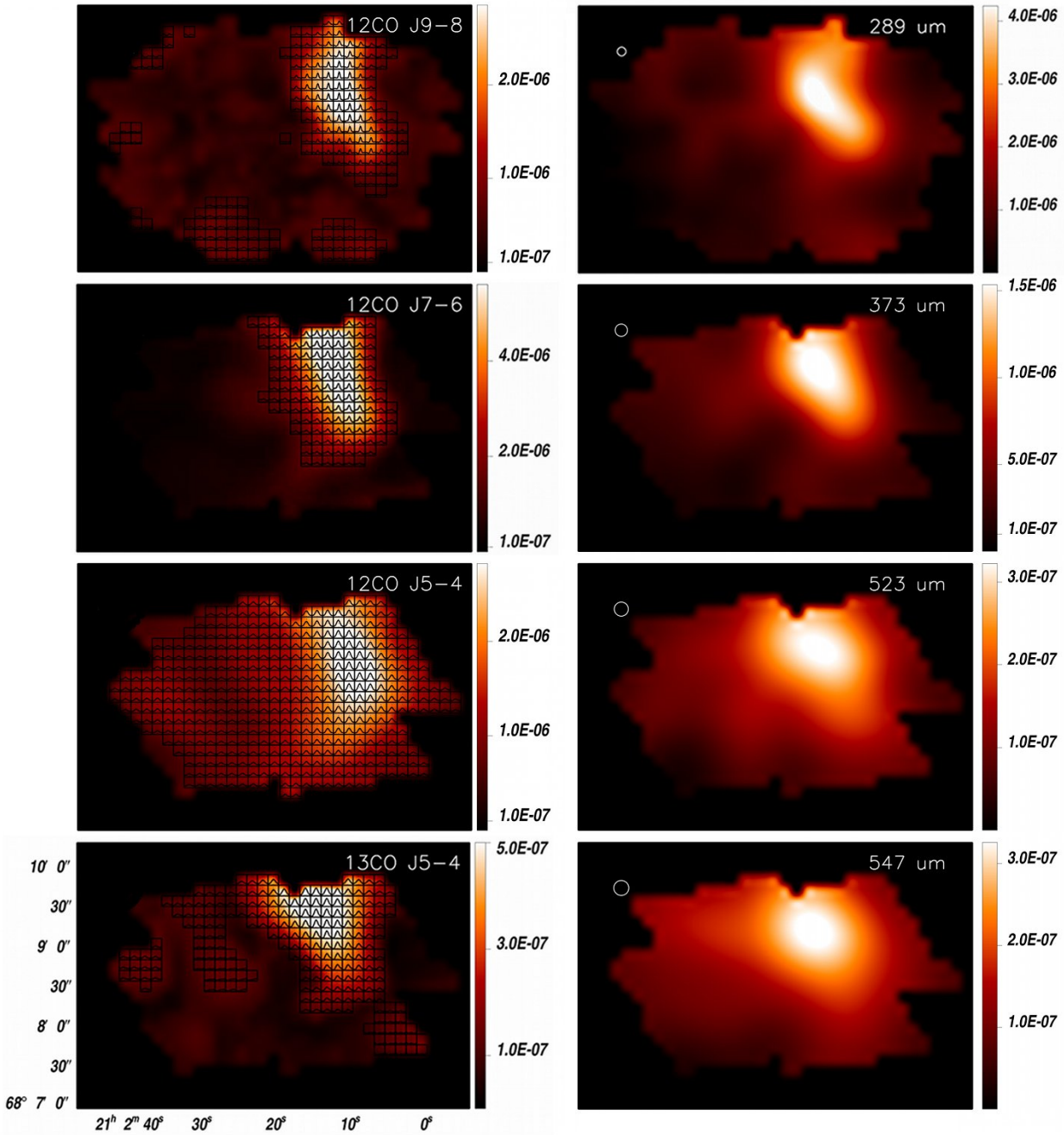
Fig. 8. Left column: Spatial distribution of ^{12}\text{CO} (J=9-8), ^{12}\text{CO} (J=7-6), ^{12}\text{CO} (J=5-4), ^{13}\text{CO} (J=5-4) lines for NGC 7023 E. The bars indicate intensities in \text{erg s}^{-1}\text{cm}^{-2}\text{sr}^{-1} . Right column: Spatial dust distribution at the wavelength close to the line emission. The bars give \nu I_\nu in \text{Wm}^{-2}\text{sr}^{-1} . All images are presented with the same scale, field, and centre. We include the FWHM of the beam in the dust emission maps: 13.0'' , 18.6'' , 21.3'' , 22.7'' from top to bottom.
