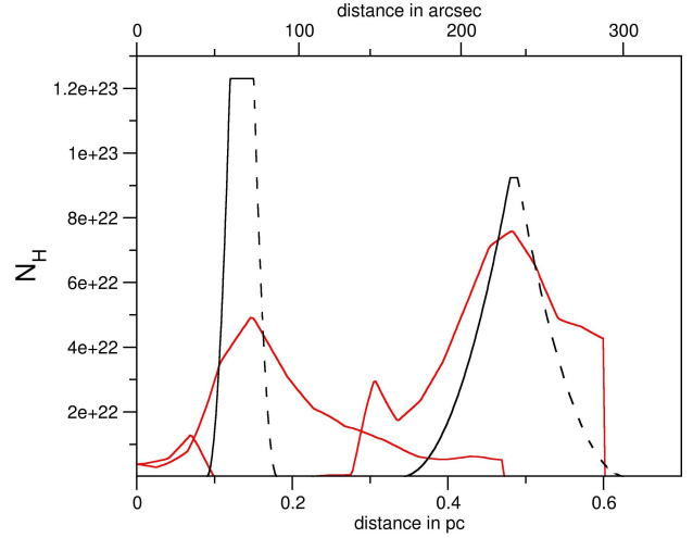
Fig. 14. The H column density profiles for NGC 7023 NW (left curves) and NGC 7023 E (right curves) derived with the blackbody approach (red curves) and the radiative transfer calculations (black curves). Since the slope of the decreasing density is ambiguous, we present it as a dashed line.
